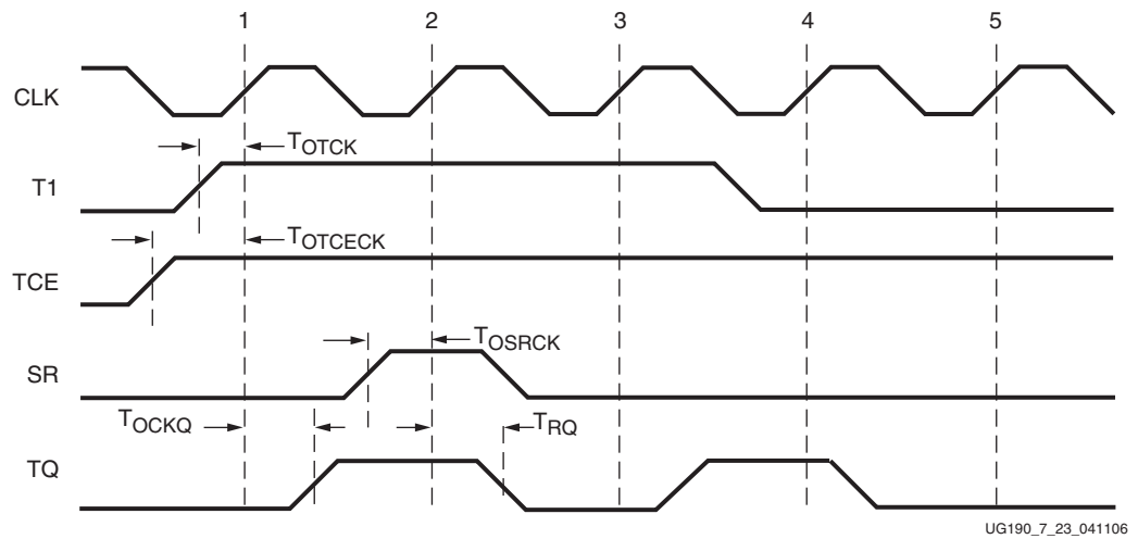
Figure 7-23: OLOGIC 3-State Register Timing Characteristics
