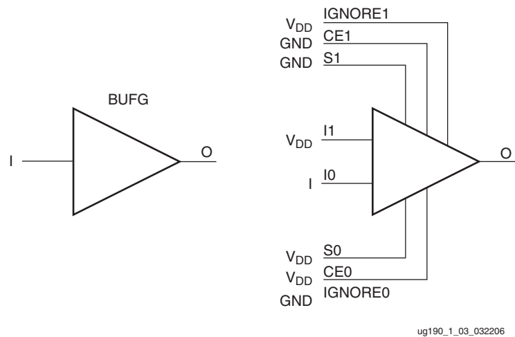
Figure 1-3: BUF as BUFCTRL
