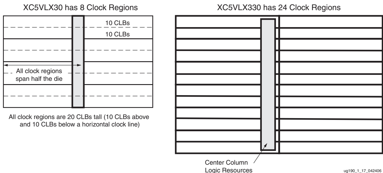
Figure 1-17: Clock Regions
