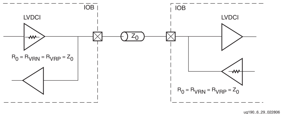
Figure 6-31: Controlled Impedance Driver with Bidirectional Termination
