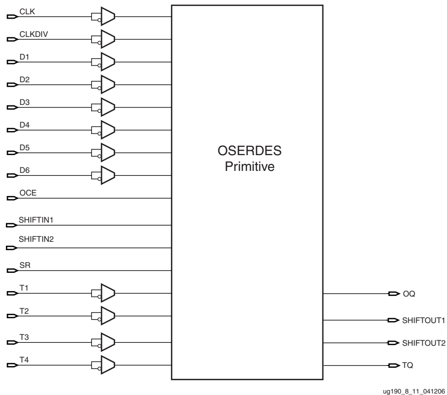
Figure 8-11: OSERDES Primitive
