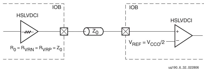
Figure 6-34: HSLVDCI Controlled Impedance Driver with Unidirectional Termination
