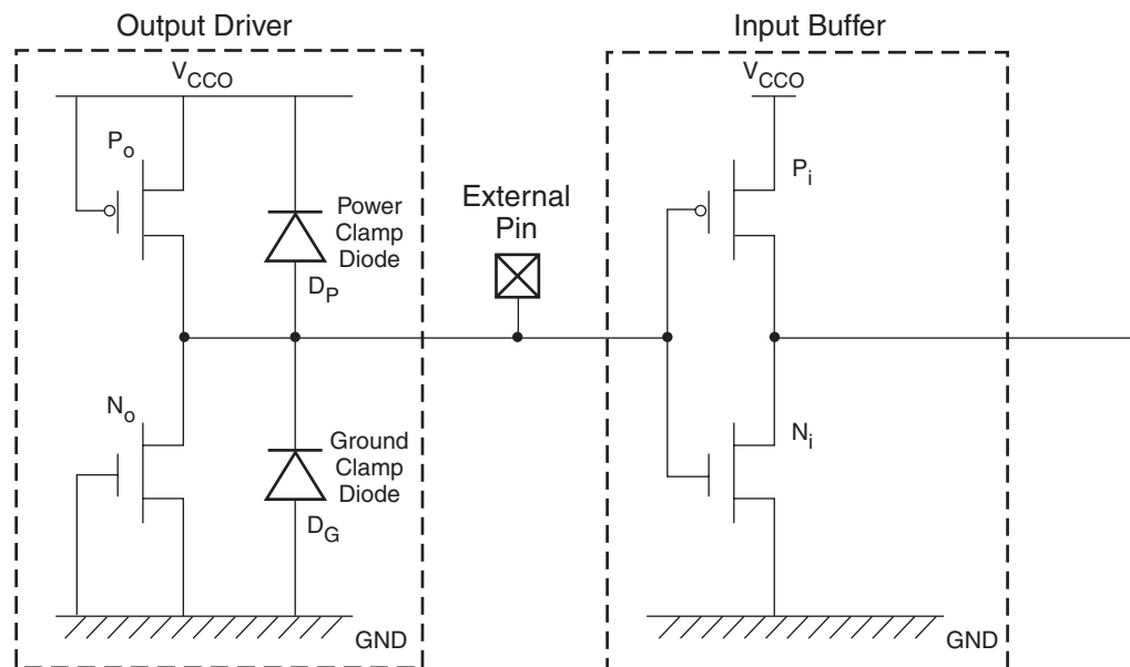
Figure 6-91: Virtex-5 I/O: 3-State Output Driver
