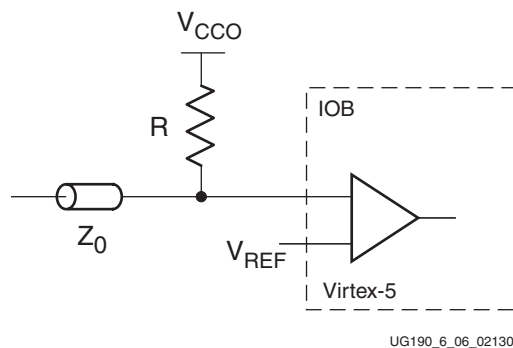
Figure 6-8: Input Termination to V_{CC0} without DCI
