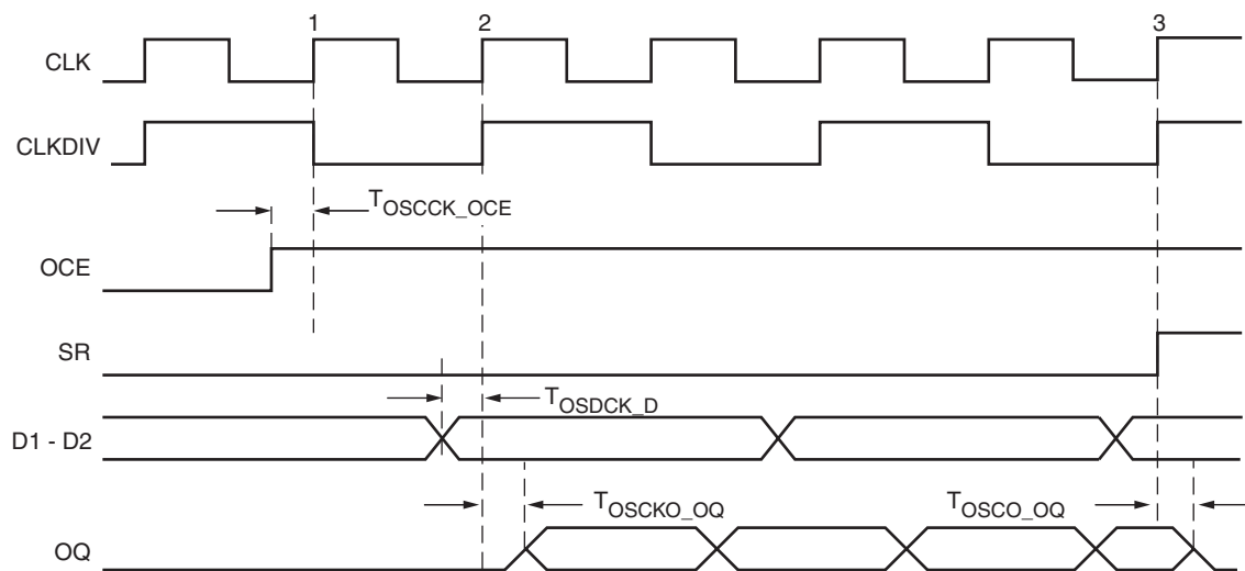
Figure 8-13: OSERDES 2:1 SDR Data Serialization Timing Diagram
