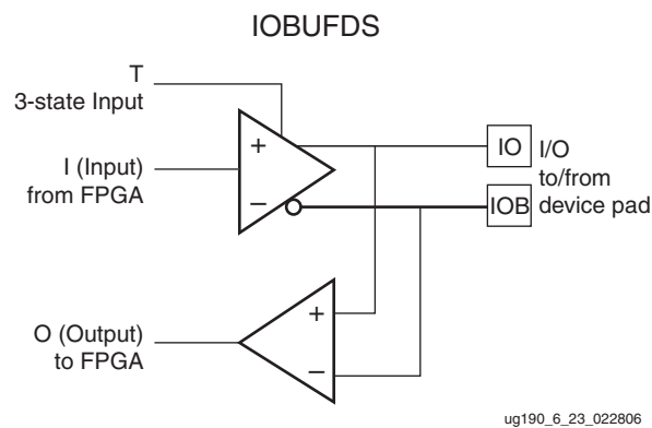
Figure 6-25: Differential Input/Output Buffer Primitive (IOBUFDS)
