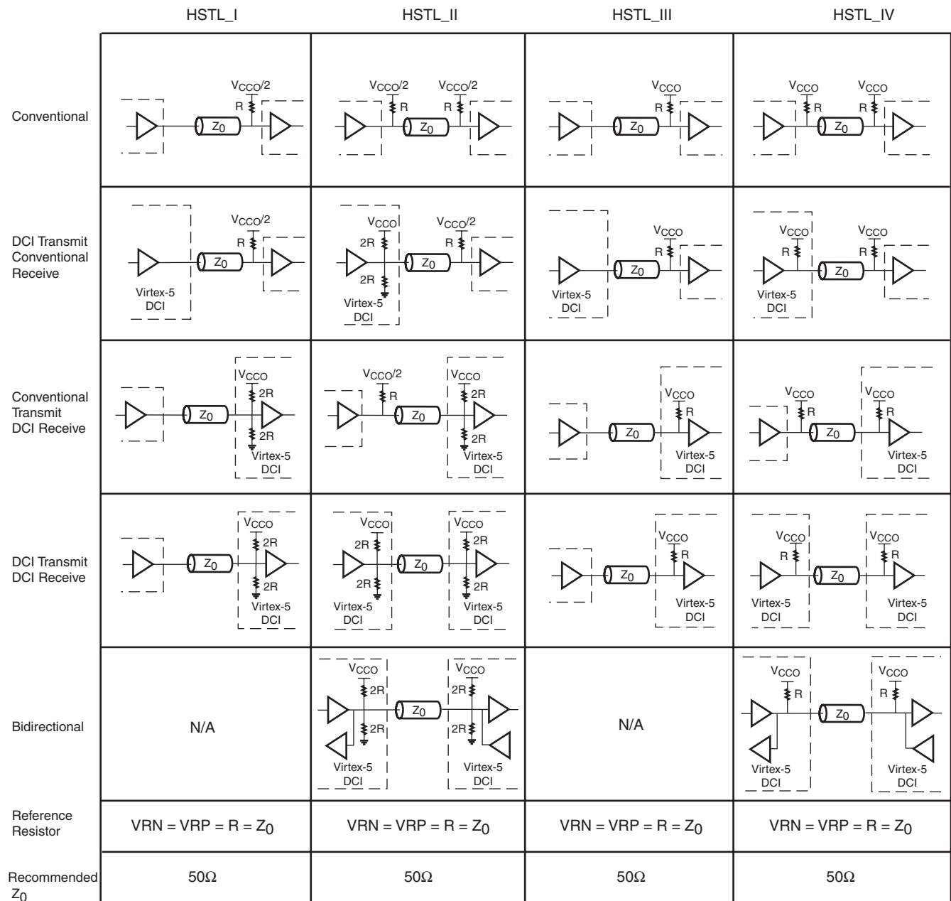
Figure 6-16: HSTL DCI Usage Examples
