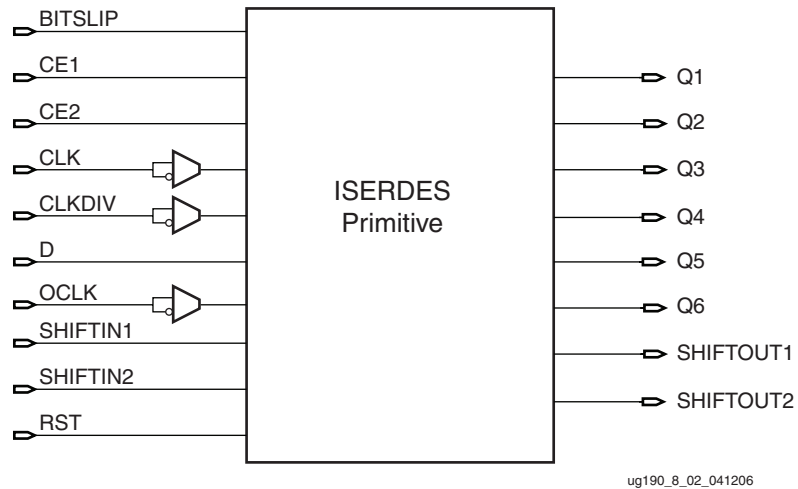
Figure 8-2: ISERDES Primitive
