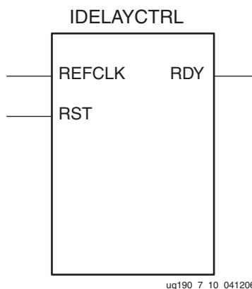
Figure 7-10: IDELAYCTRL Primitive
