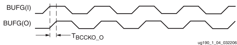
Figure 1-4: BUF Timing Diagram
