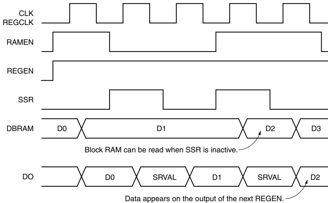
Figure 4-12: SSR Operation in Register Mode with REGEN High
