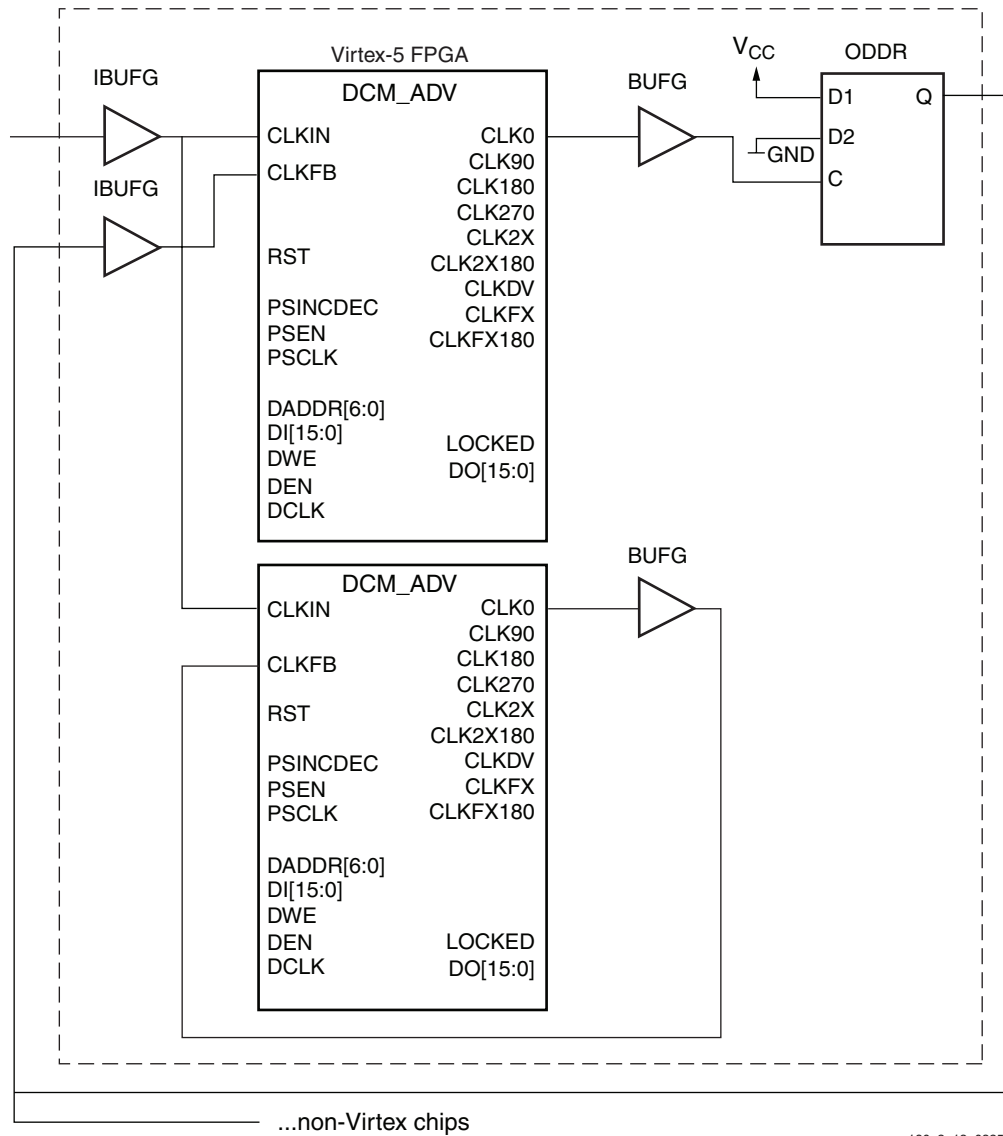
Figure 2-13: Board Deskew with Internal Deskew Interfacing to Other Components
