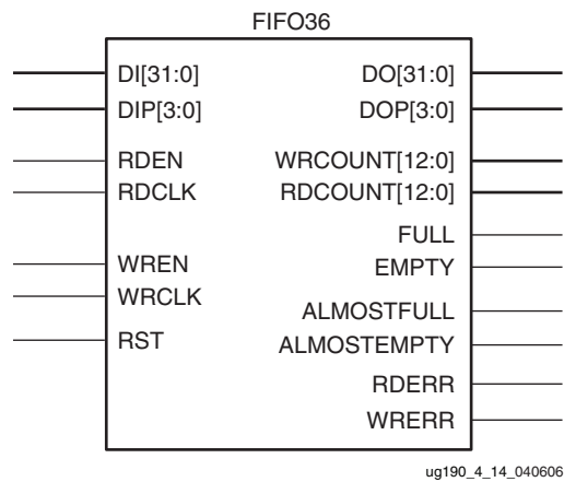
Figure 4-17: FIFO36 Primitive
