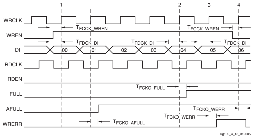
Figure 4-21: Writing to a Full / Almost Full FIFO
