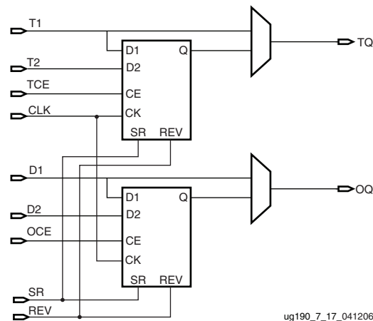
Figure 7-17: OLOGIC Block Diagram
