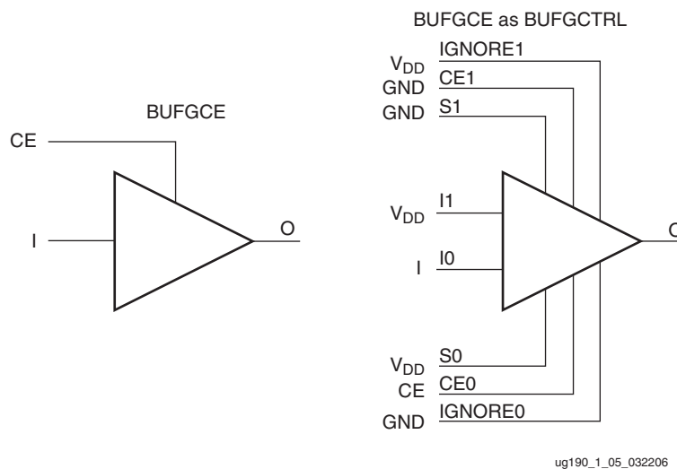
Figure 1-5: BUFGE as BUFCTRL
