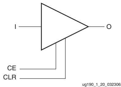
Figure 1-20: BUFR Primitive
