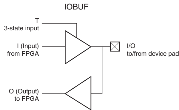
Figure 6-21: Input/Output Buffer (IOBUF) Primitive
