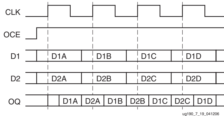
Figure 7-19: Output DDR Timing in SAME_EDGE Mode
