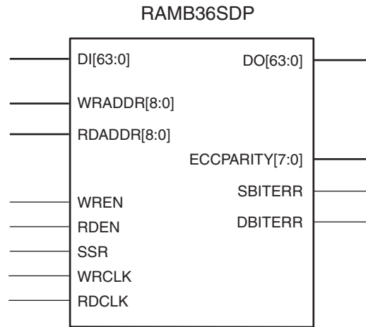
Figure 4-28: RAMB36SDP: Block RAM ECC Primitive
