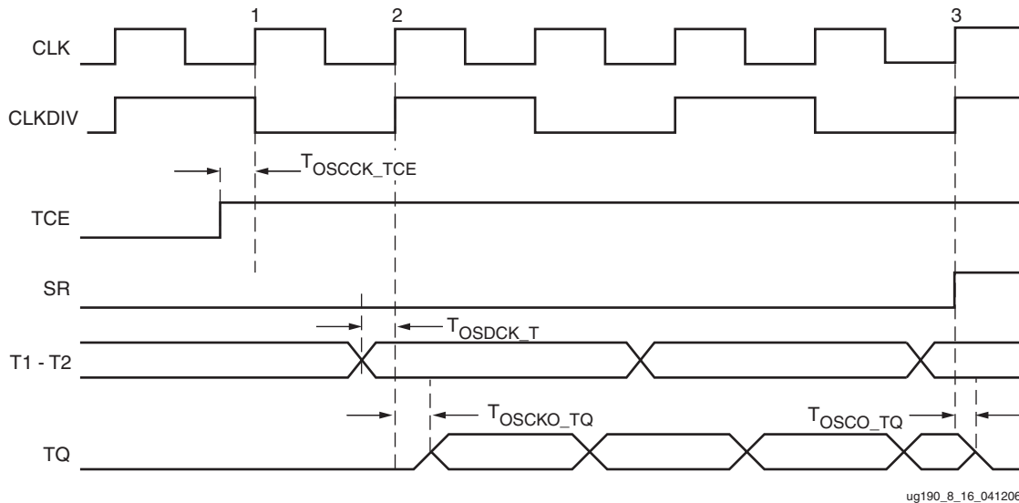
Figure 8-16: OSERDES 2:1 SDR 3-State Control Serialization Timing Diagram
