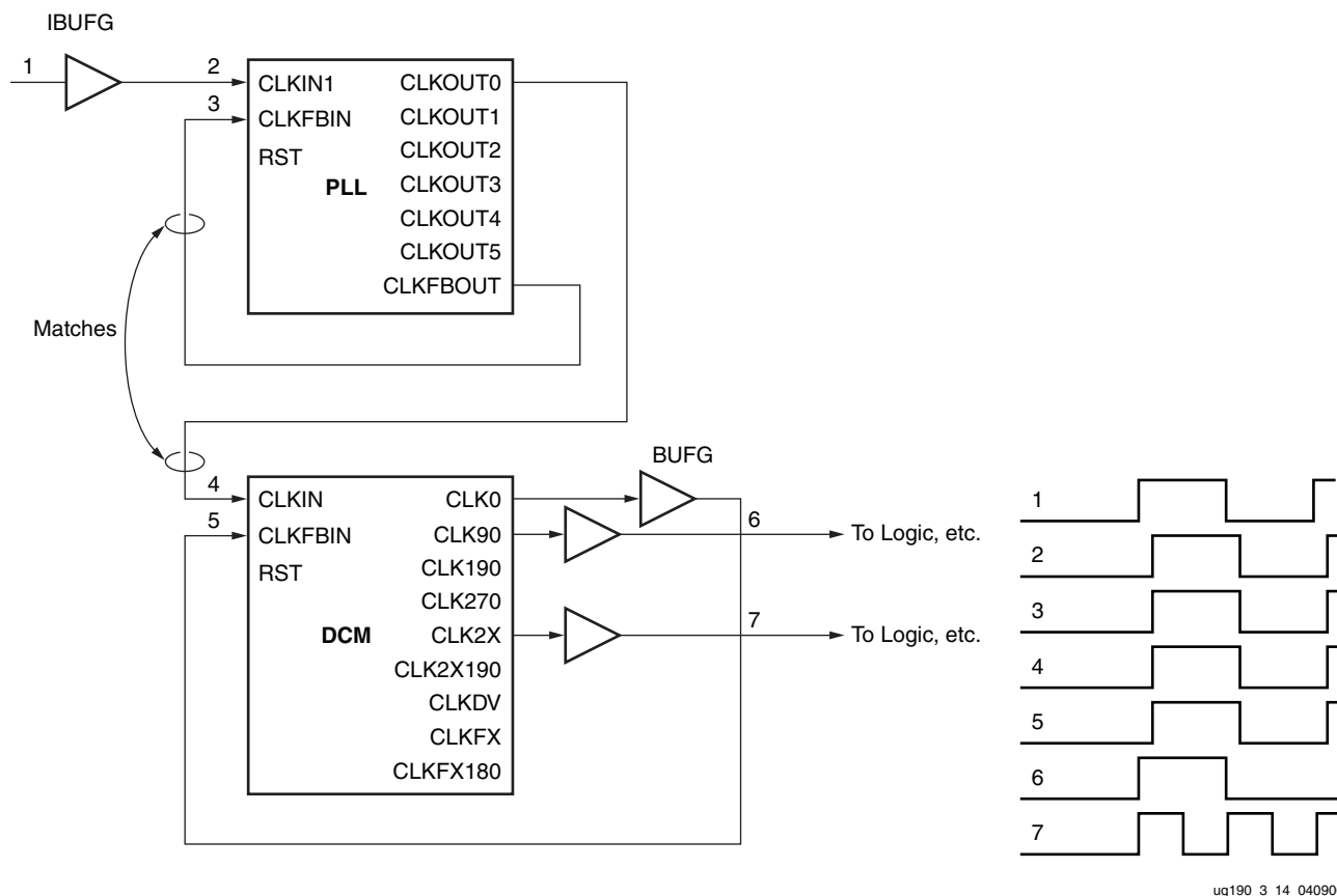
Figure 3-14: PLL Driving DCMs
