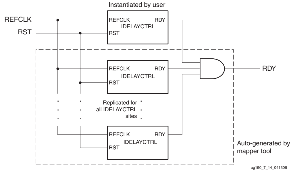
Figure 7-14: Instantiate IDELAYCTRL Without LOC Constraints - RDY Connected
