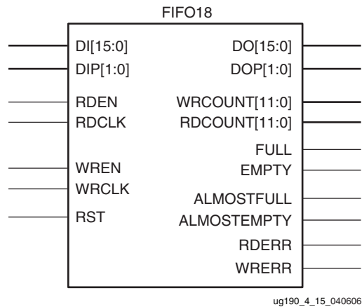
Figure 4-18: FIFO18 Primitive
