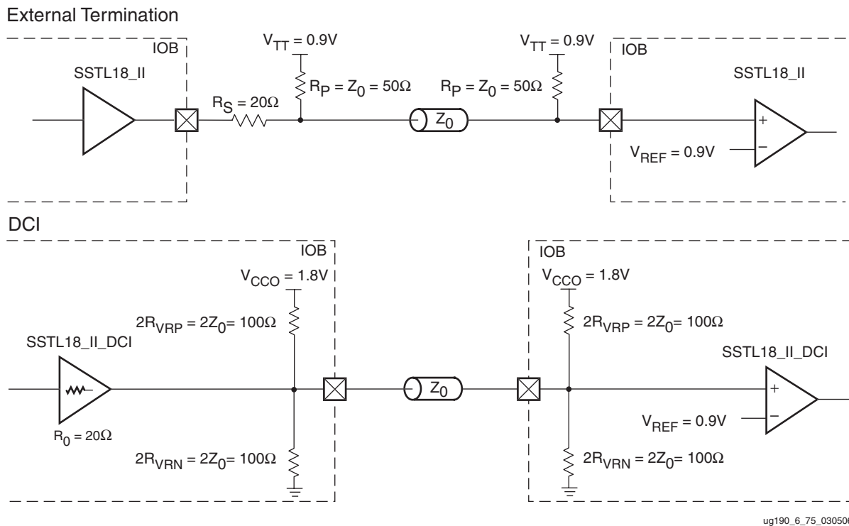
Figure 6-80: SSDL18 (1.8V) Class II Unidirectional Termination
