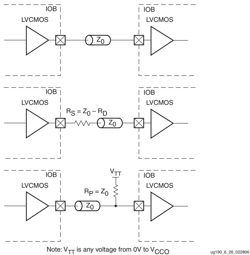
Figure 6-28: LVCMOS Unidirectional Termination
