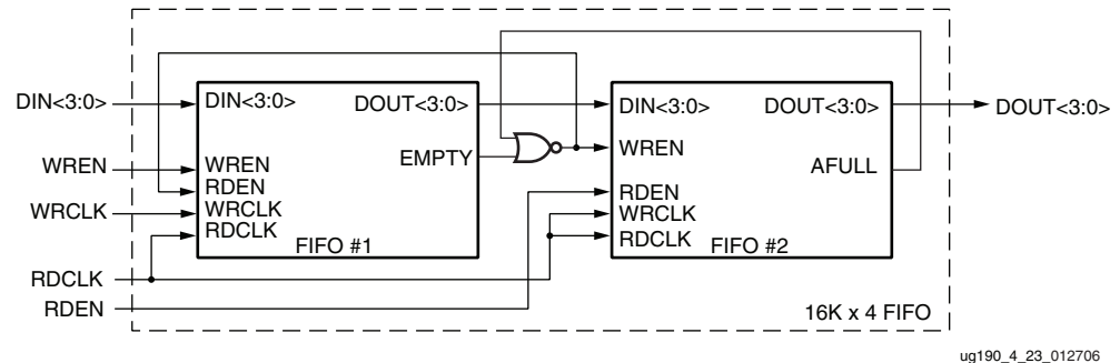
Figure 4-25: Cascading FIFO
