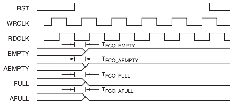
Figure 4-24: Resetting All Flags
