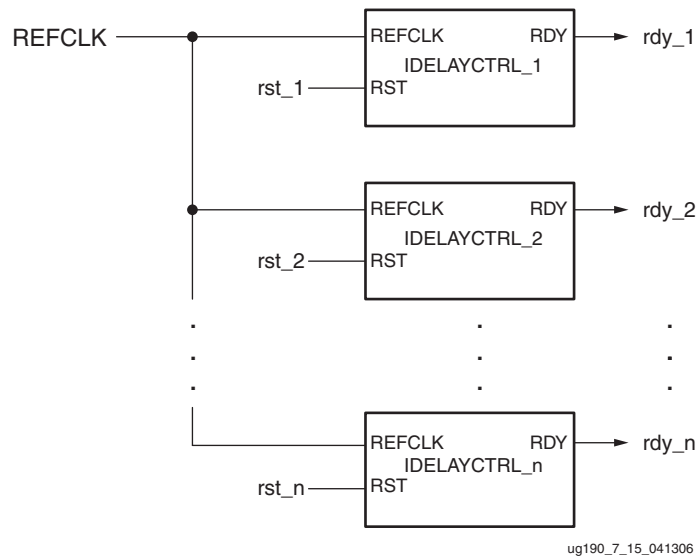
Figure 7-15: Instantiate IDELAYCTRL with LOC Constraint
