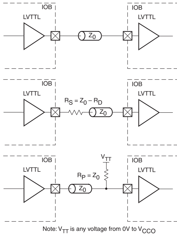
Figure 6-26: LVTTL Unidirectional Termination
