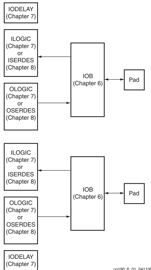
Figure 6-1: Virtex-5 I/O Tile
