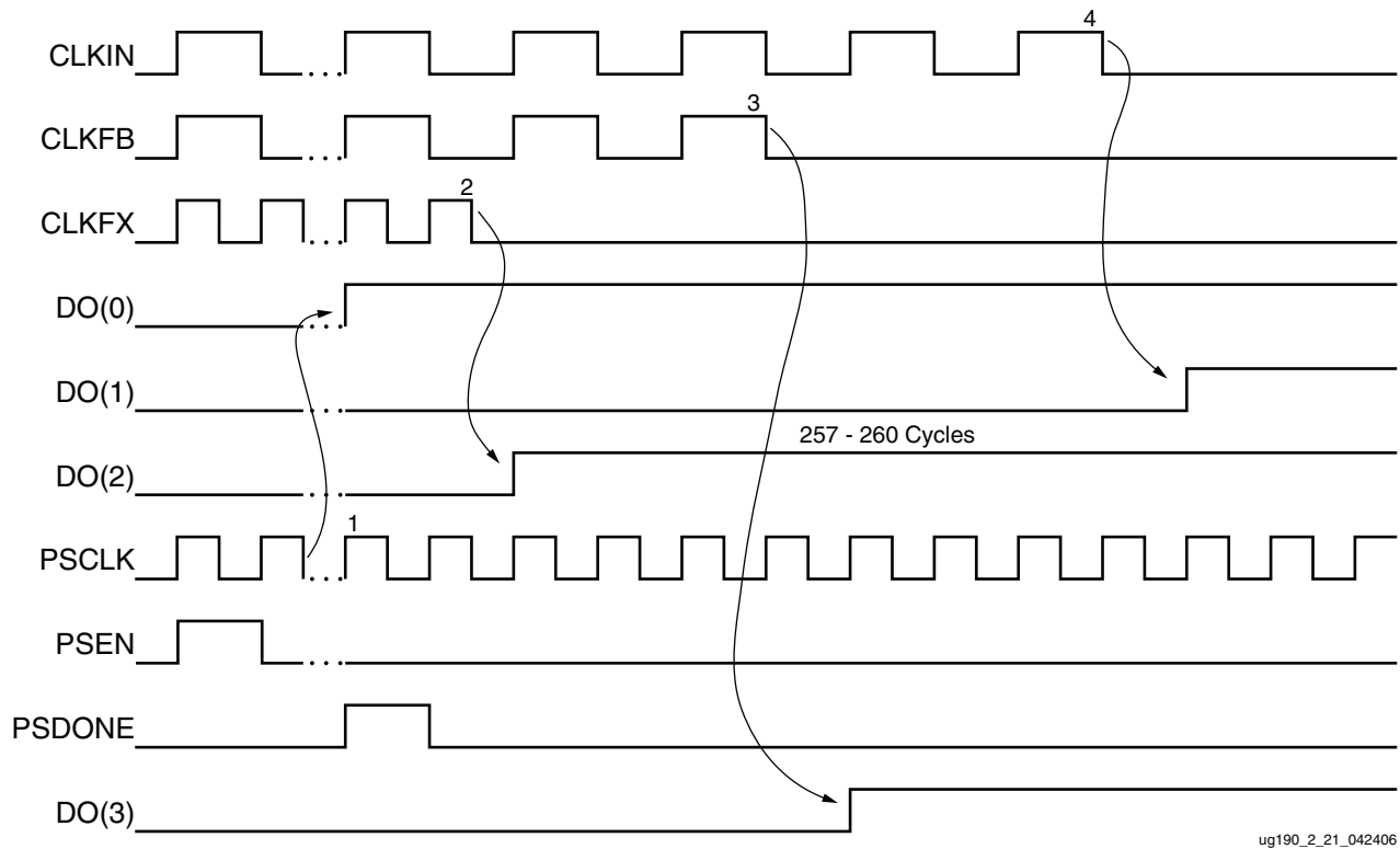
Figure 2-21: Status Flags Example
