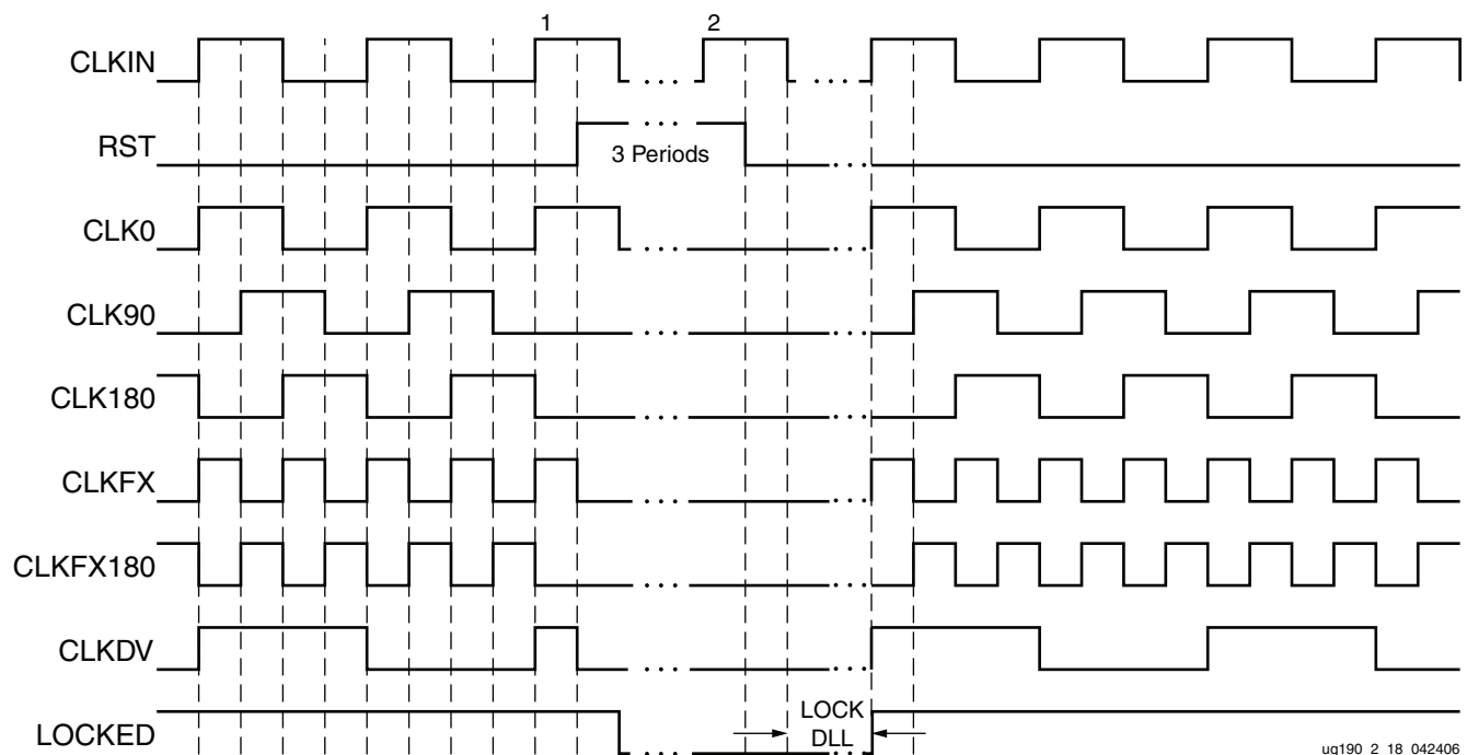
Figure 2-18: RESET/LOCK Example
