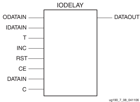
Figure 7-8: IODELAY Primitive
