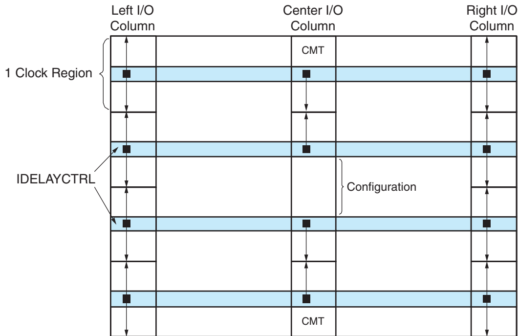
Figure 7-12: Relative Locations of IDELAYCTRL Modules
