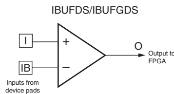
Figure 6-22: Differential Input Buffer Primitive (IBUFDS/IBUFGDS)
