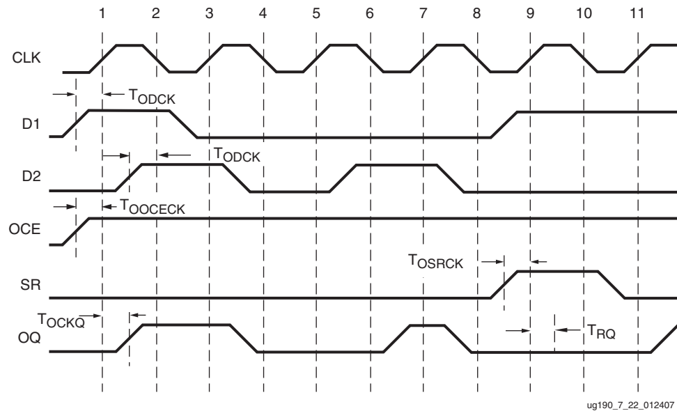
Figure 7-22: OLOGIC ODDR Register Timing Characteristics
