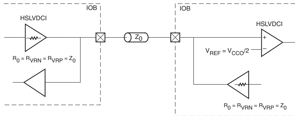
Figure 6-35: HSLVDCI Controlled Impedance Driver with Bidirectional Termination
