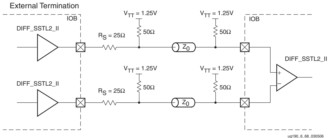
Figure 6-72: Differential SSTL2 Class II Unidirectional Termination
