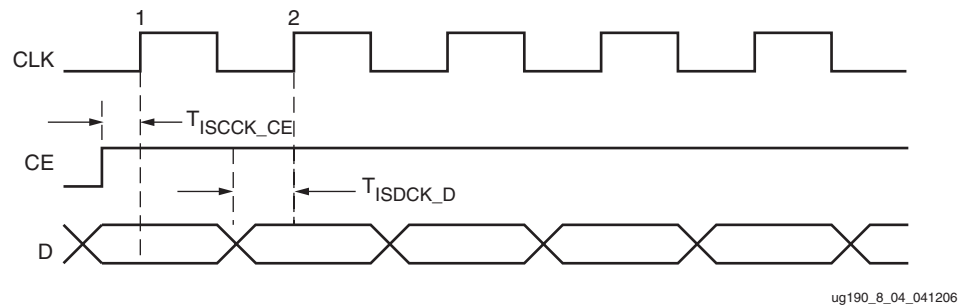
Figure 8-4: ISERDES Input Data Timing Diagram
