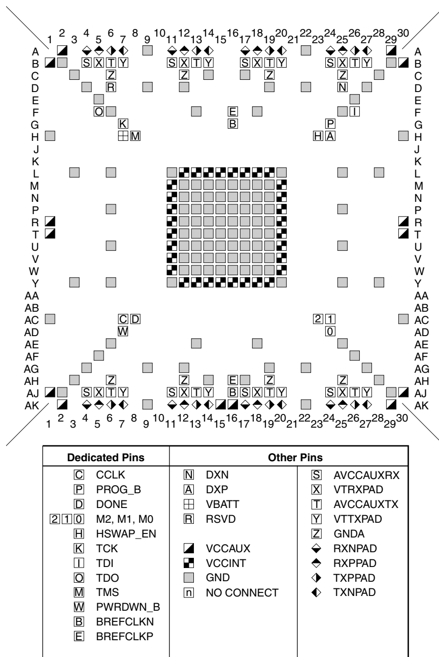
Figure 5-31: FF896 Dedicated/Other Pins (XC2VPX20)
