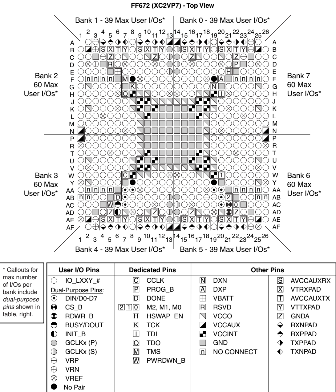
Figure 5-16: FF672 Flip-Chip Fine-Pitch BGA Composite Pinout Diagram
