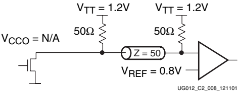
Figure 3-82: GTL Terminated
