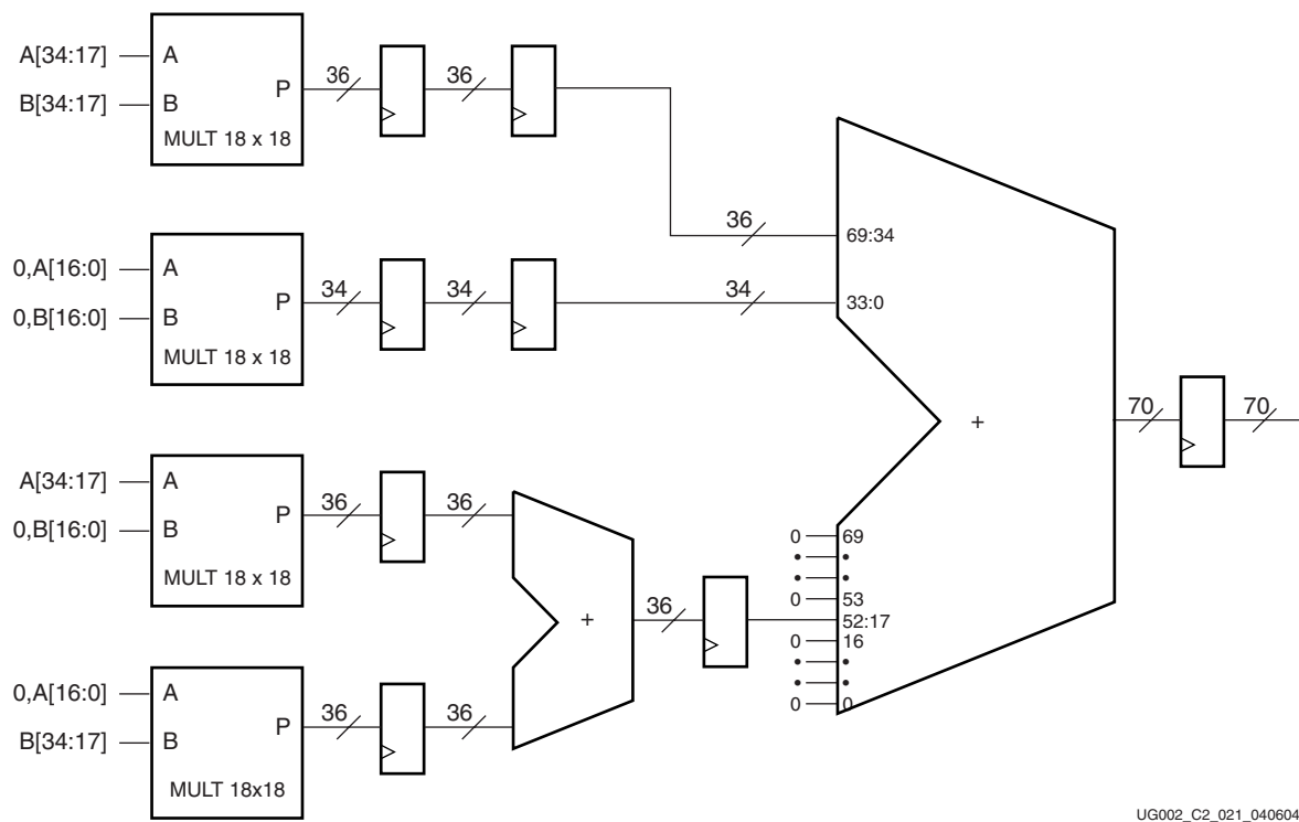
Figure 3-71: MULT35X35_S Submodule
