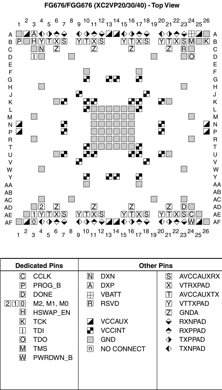
Figure 5-15: FG676/FGG676 Dedicated/Other Pins (XC2VP20, XC2VP30, XC2VP40)
