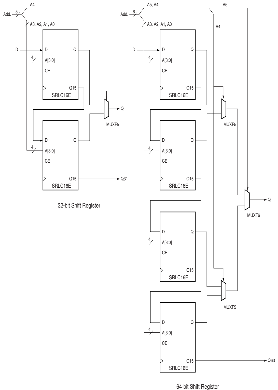
Figure 3-57: Shift-Register Submodules (32-bit, 64-bit)
