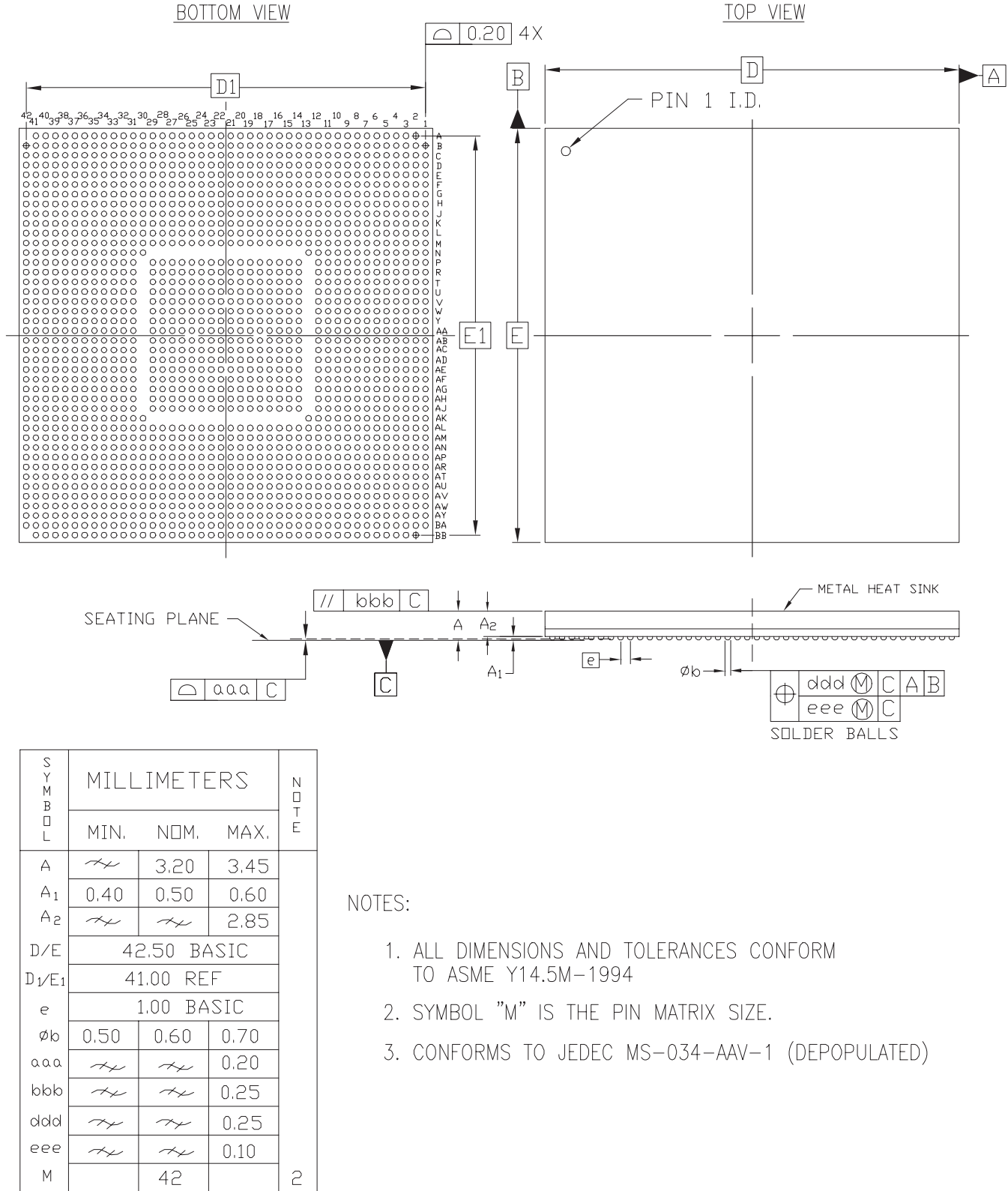
Figure 5-73: FF1696 Flip-Chip Fine-Pitch BGA Package
