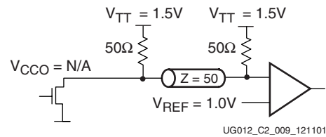
Figure 3-83: GTLP Terminated
