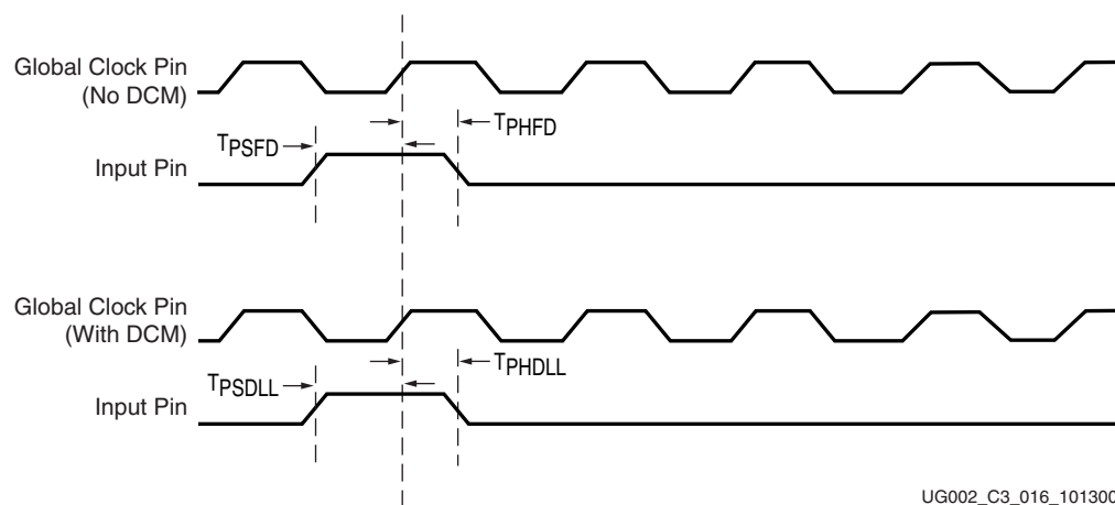
Figure 2-25: Global Clock Setup and Hold Timing Characteristics
