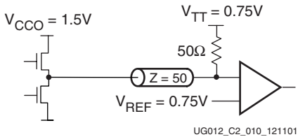
Figure 3-84: Terminated HSTL Class I
