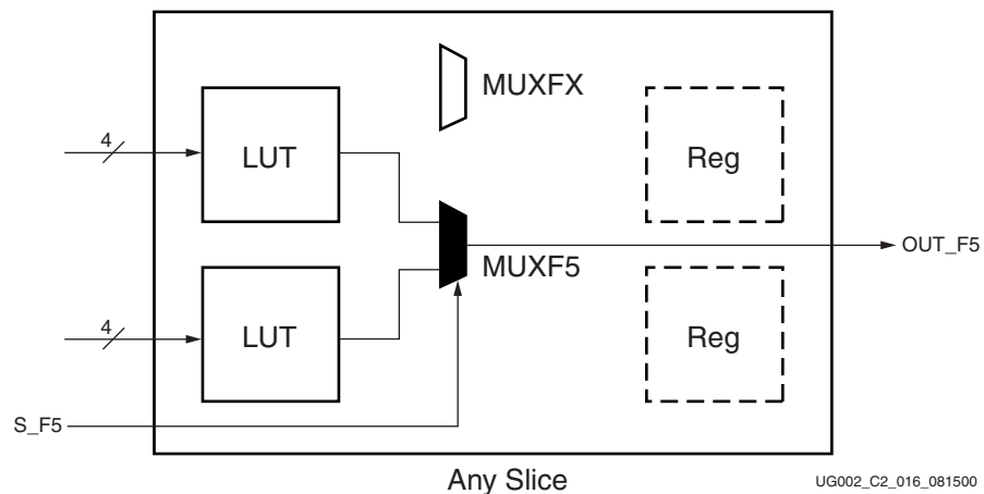
Figure 3-61: LUTs and MUXF5 in a Slice
