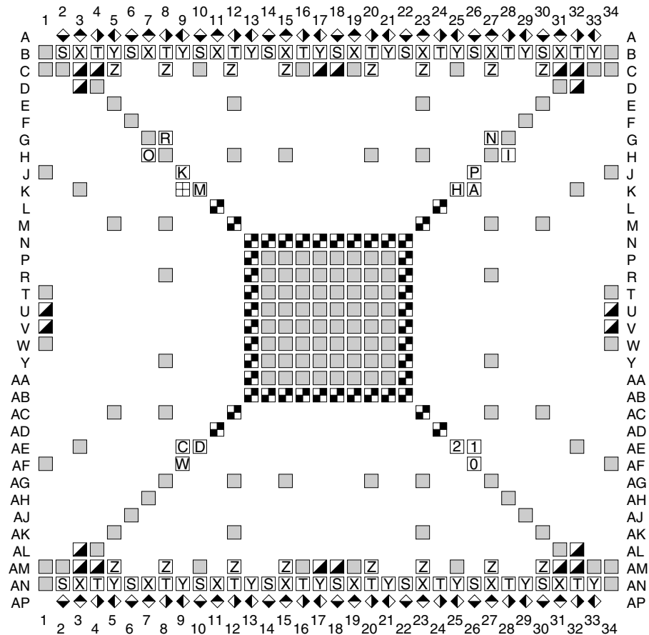
FF1152 (XC2VP50) - Top View
