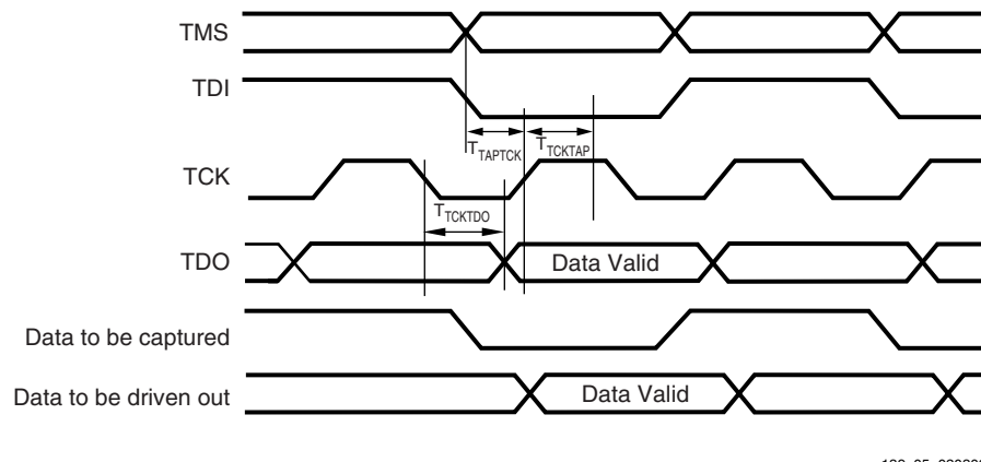
Figure 4-25: Virtex-II Pro Boundary Scan Port Timing Waveforms
