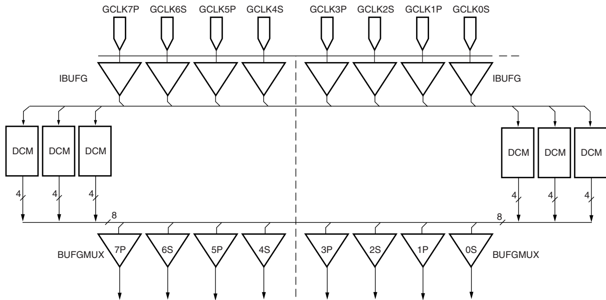
Figure 3-10: DCM Clocks
