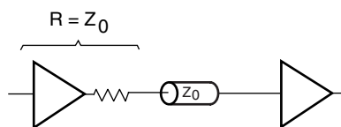
Figure 5-78: Series Termination
