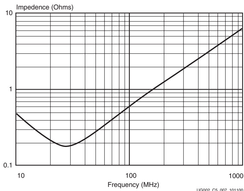
Figure 5-75: 33000 pF X7R Component Frequency Response Curve
