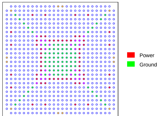
Figure 5-79: Fine-Pitch BGA Pin Assignments
