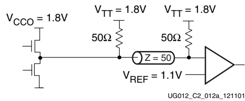
Figure 3-91: Terminated HSTL Class IV (1.8V)
