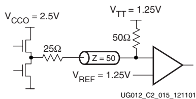
Figure 3-92: Terminated SSTL2_I
