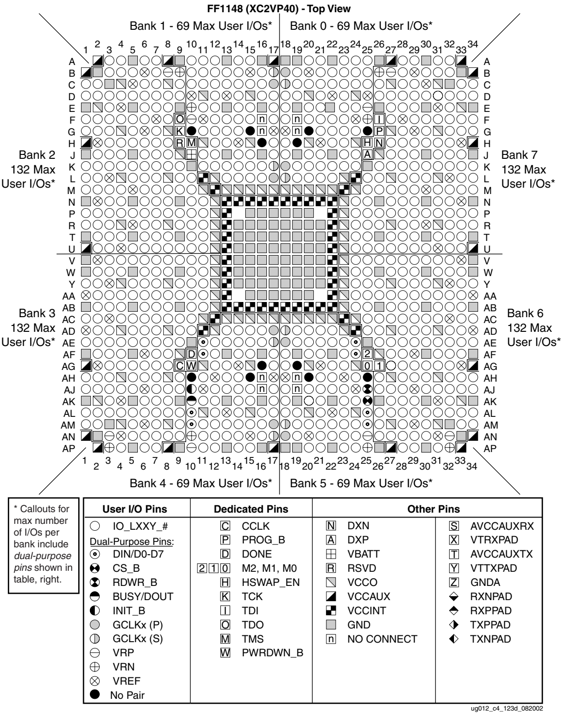
Figure 5-45: FF1148 Composite Pinout Diagram (XC2VP40)
