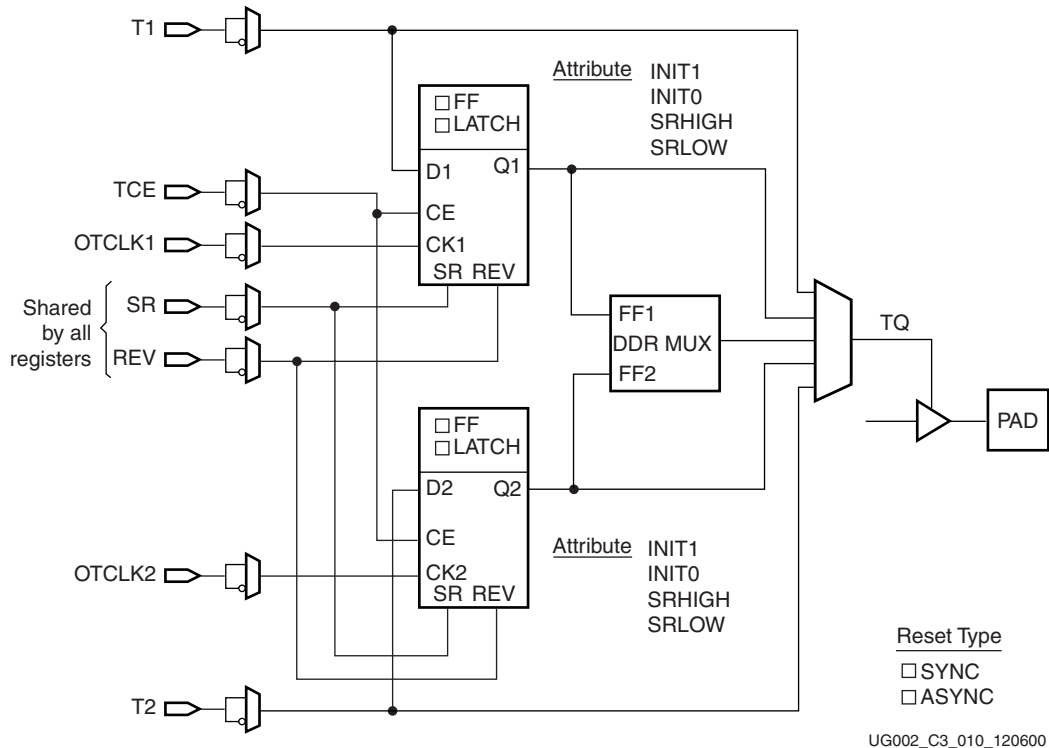
Figure 2-19: Virtex-II Pro/Virtex-II Pro X IOB 3-State
