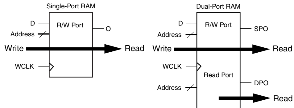
Figure 3-49: Single-Port and Dual-Port Distributed SelectRAM
