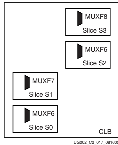
Figure 3-62: Slice Positions in a CLB
