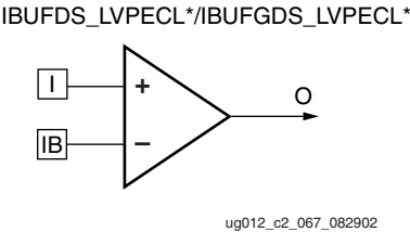
Figure 3-123: LVPECL Input and Clock Primitives
