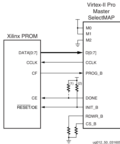
Figure 4-12: Single-Device Master SelectMAP Configuration
