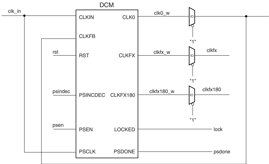
Figure 3-35: BUFG_PHASE_CLKFX_FB_SUBM
