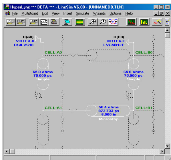
Figure 5-87: DCI Driver Example
