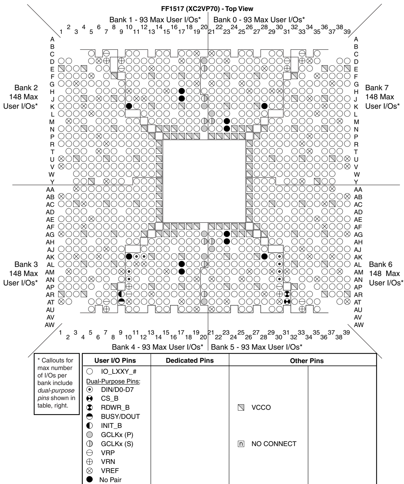
Figure 5-49: FF1517 Banked Pins (XC2VP70)
