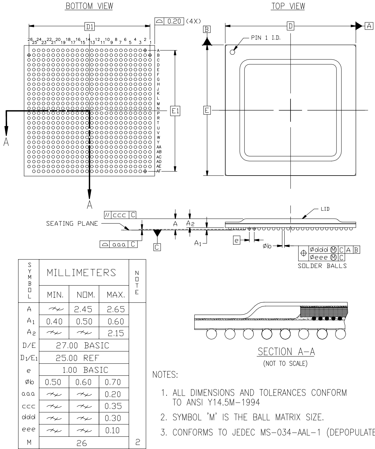
Figure 5-67: FF672 Flip-Chip Fine-Pitch BGA Package
