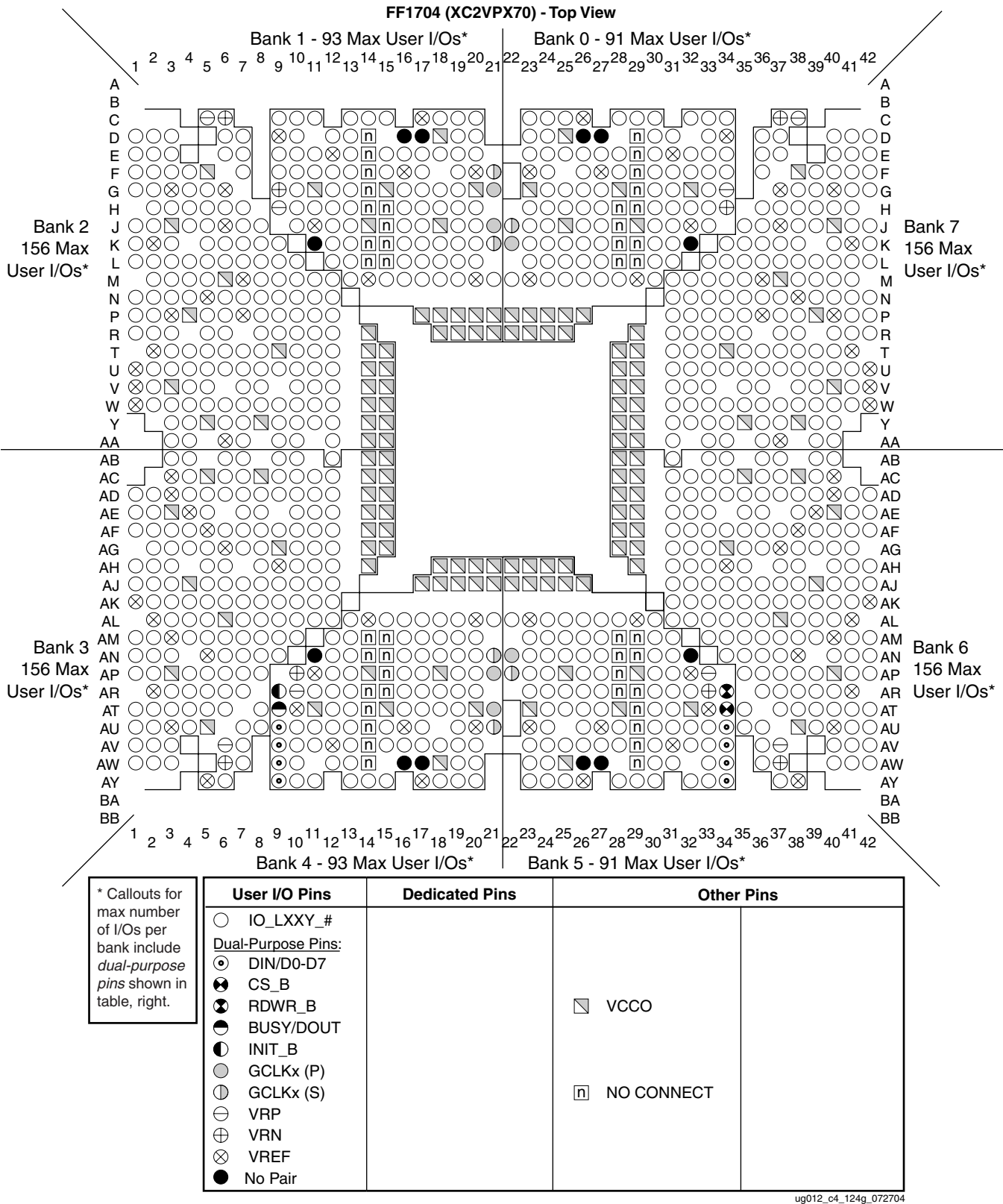
Figure 5-59: FF1704 Composite Pinout Diagram (XC2VPX70)
