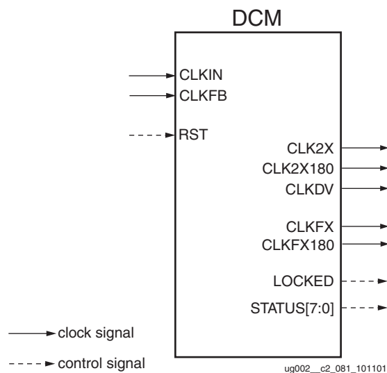
Figure 3-27: Frequency Synthesis Outputs
