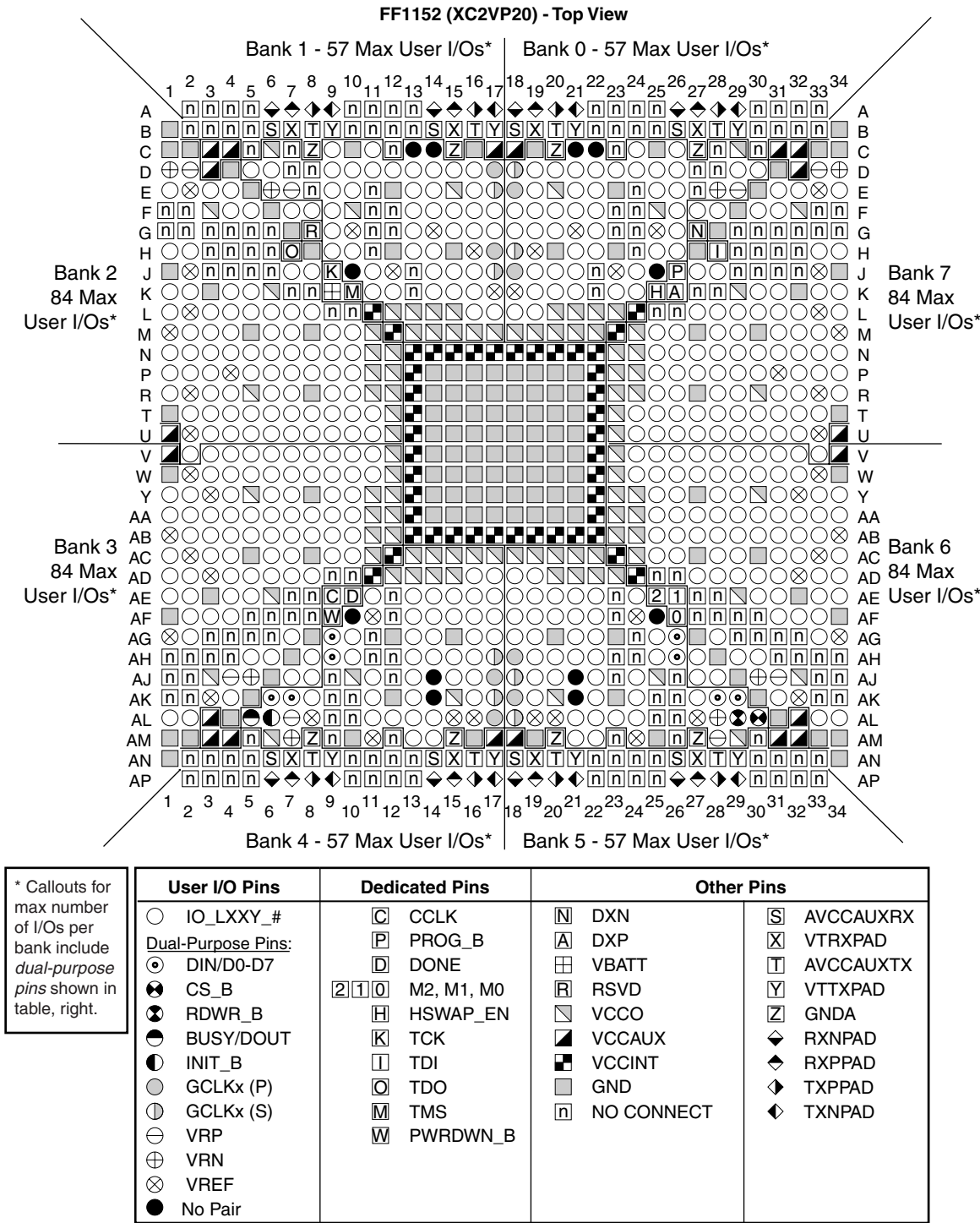
Figure 5-40: FF1152 Composite Pinout Diagram (XC2VP20)
