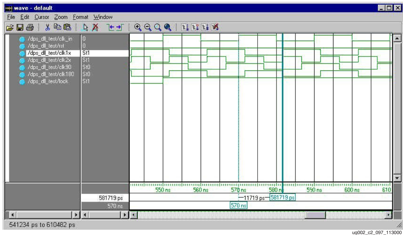
Figure 3-40: DCM_DPS Waveforms
