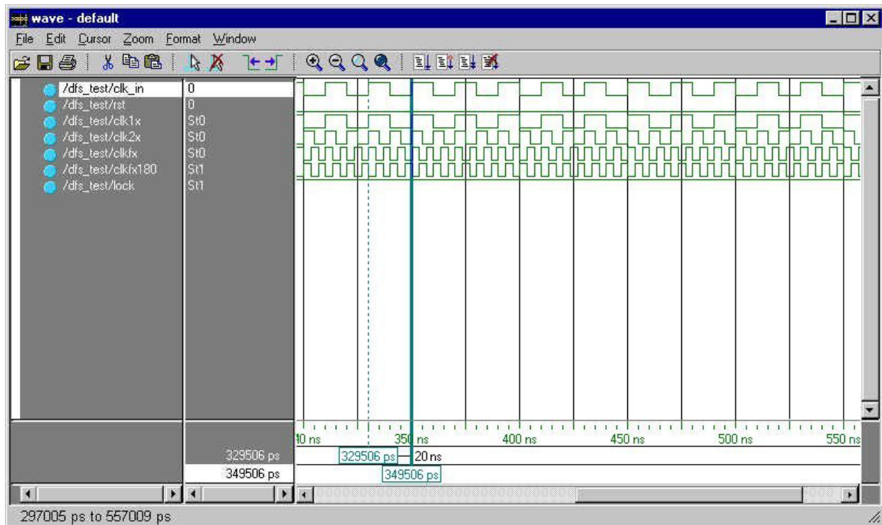
Figure 3-39: DCM_DFS Waveforms
