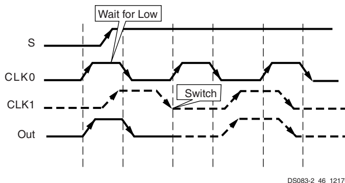
Figure 3-17: BUFGMUX Waveform Diagram
