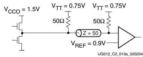
Figure 3-89: Terminated HSTL Class II (1.8V)
