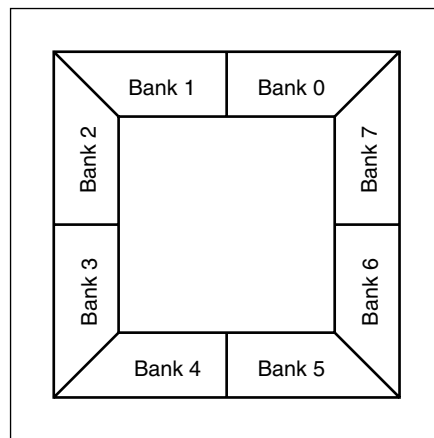
Figure 3-76: I/O Banks: Top View for Flip-Chip Packages (FF)
