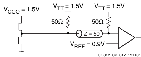
Figure 3-87: Terminated HSTL Class IV
