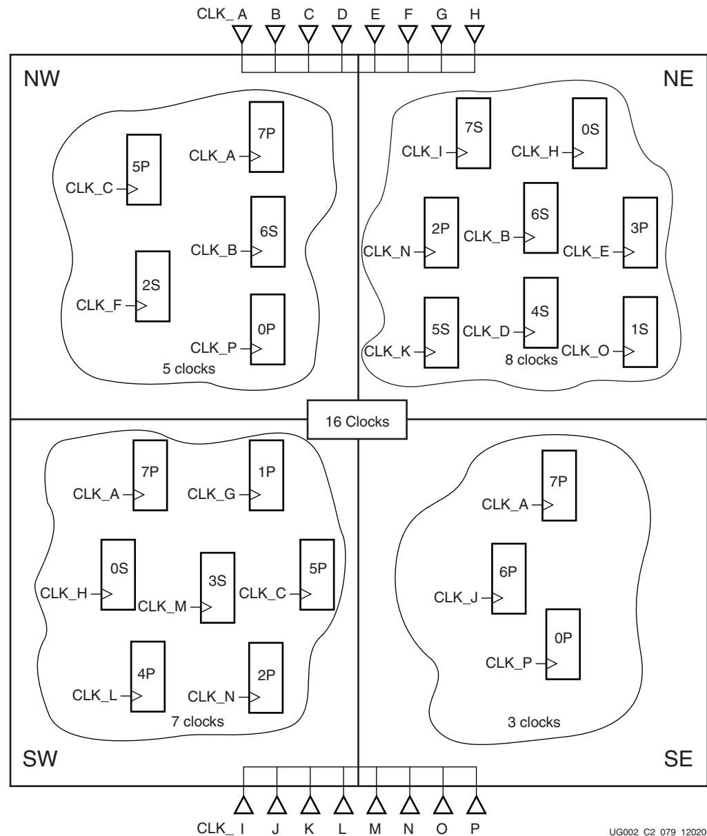
Figure 3-12: 16-Clock Floorplan
