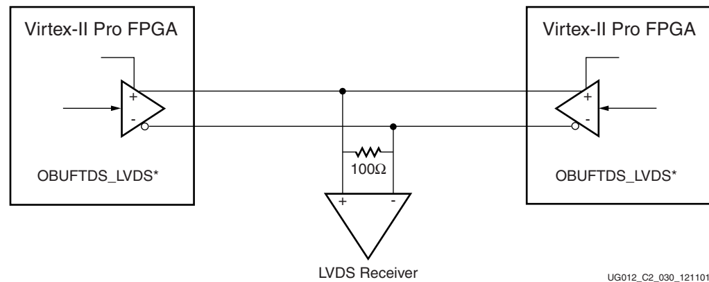
Figure 3-122: LVDS 3-State Termination
