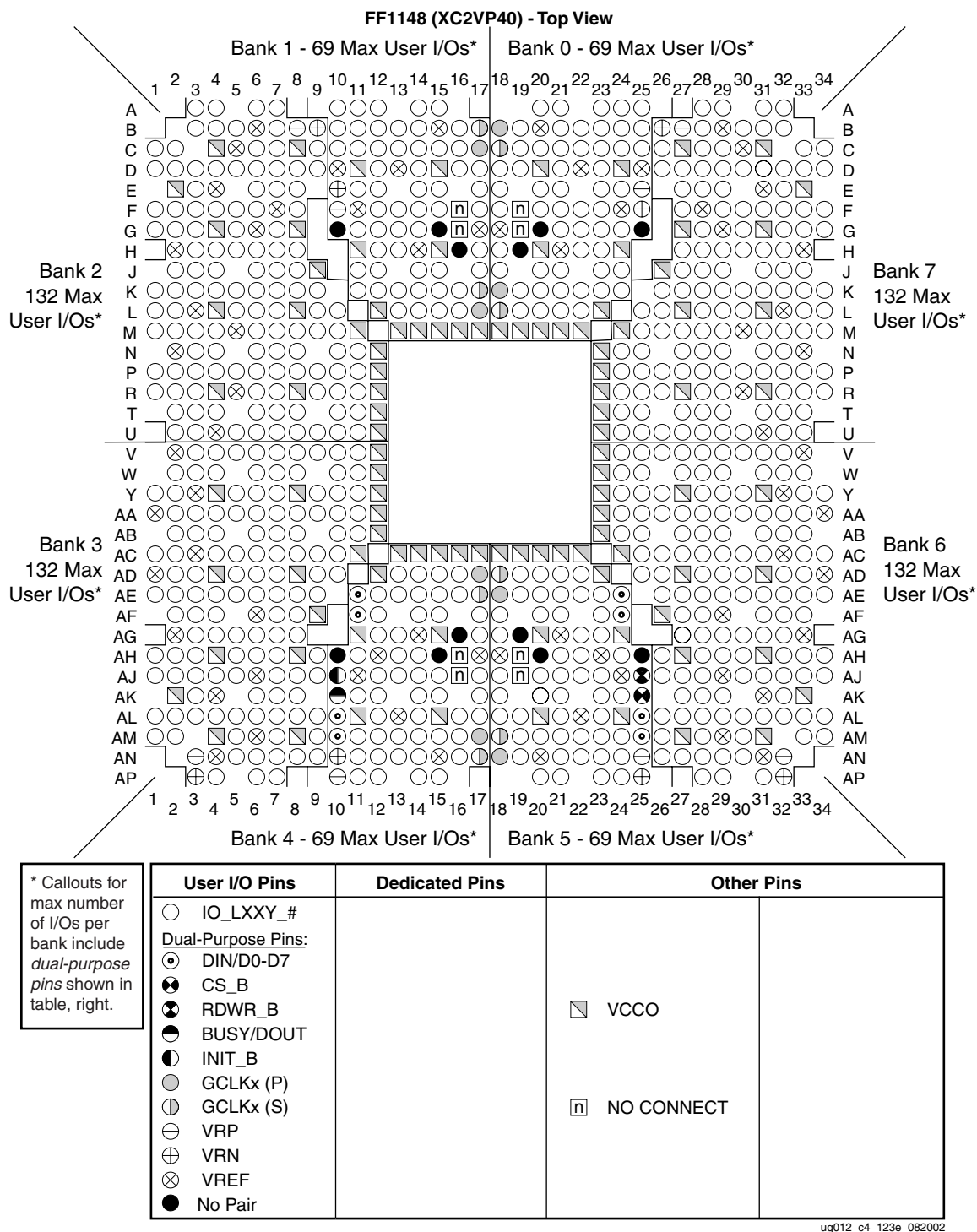
Figure 5-46: FF1148 Banked Pins (XC2VP40)
