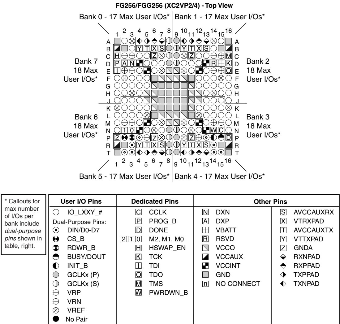
Figure 5-1: FG256/FGG256 Composite Pinout Diagram (XC2VP2, XC2VP4)
