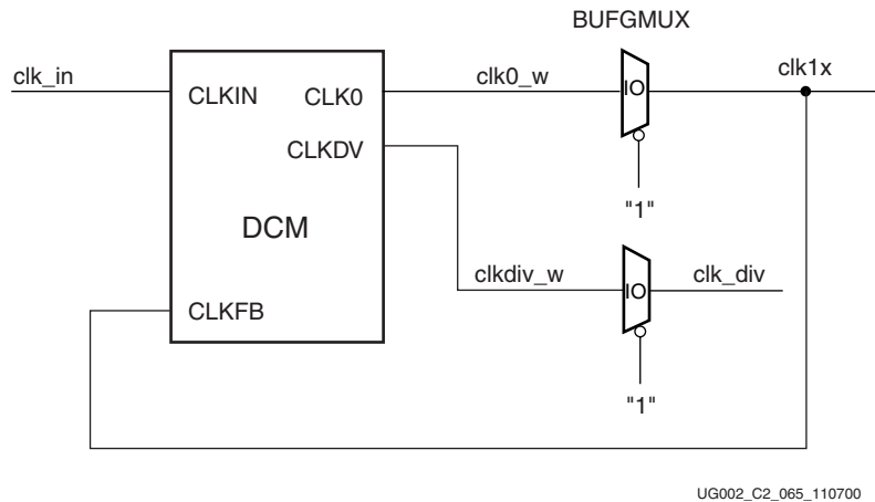
Figure 3-26: BUFG_CLKDV_SUBM
