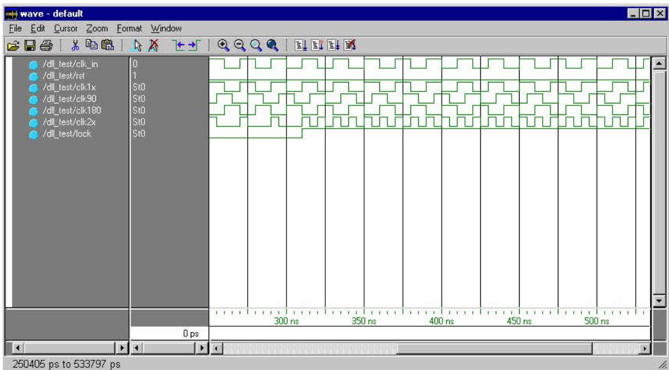
Figure 3-38: DCM_DLL Waveforms
