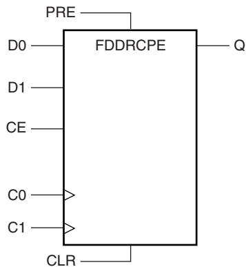
Figure 3-116: FDDRCPE Symbol: DDR Flip-Flop With Clock Enable and Asynchronous PRESET and CLR
