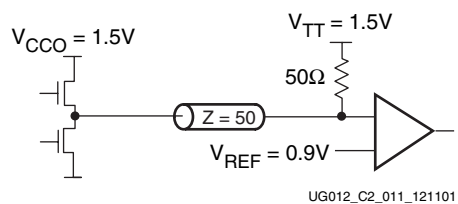
Figure 3-86: Terminated HSTL Class III
