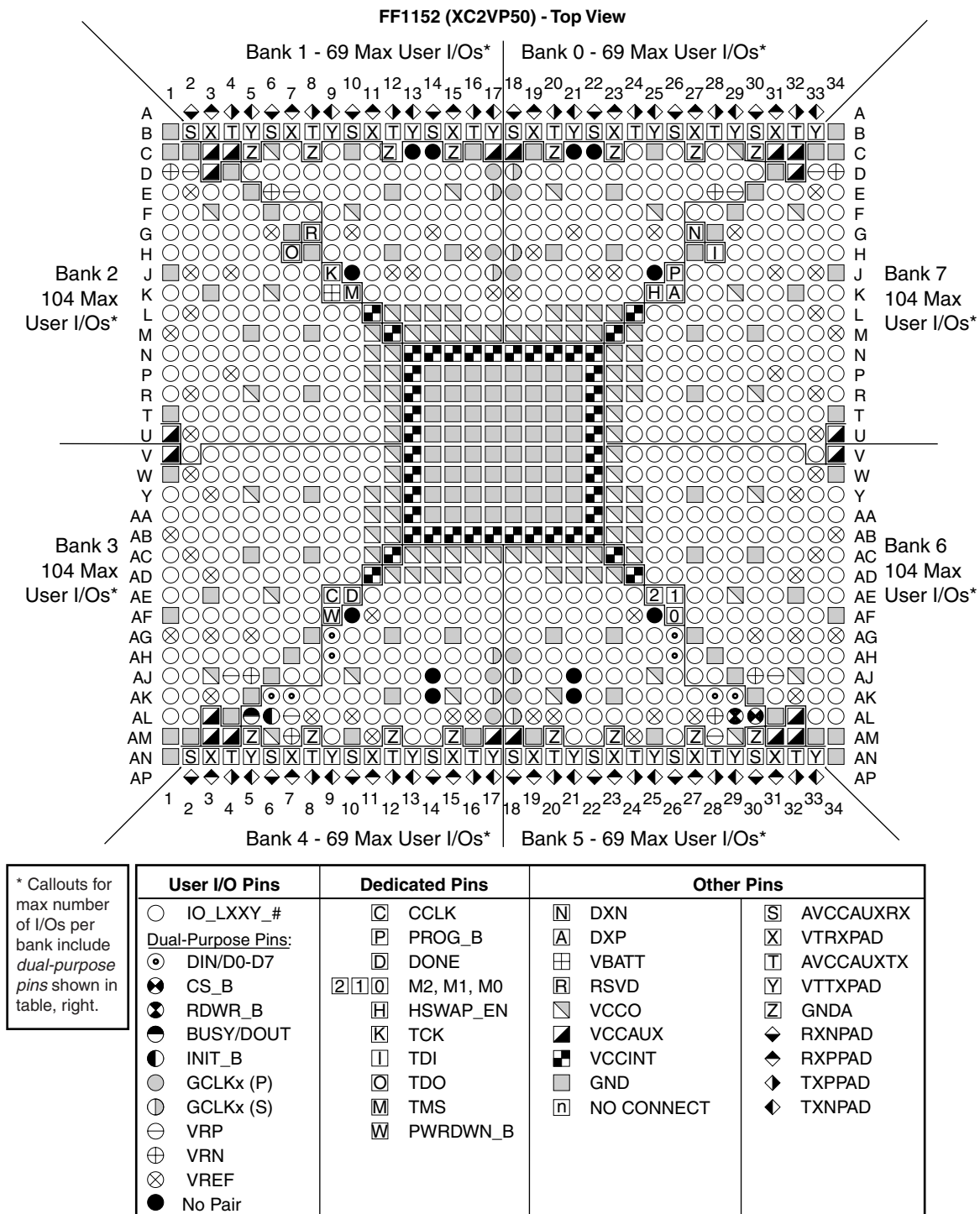
Figure 5-32: FF1152 Composite Pinout Diagram (XC2VP50)
