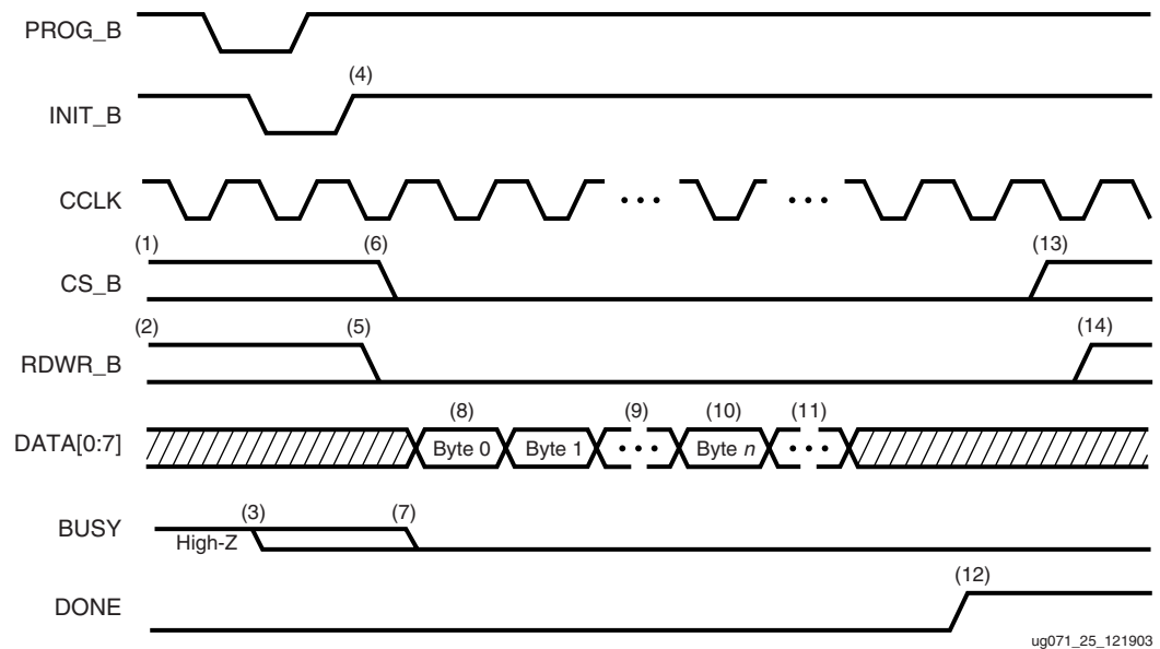
Figure 4-15: Continuous Data Loading for SelectMAP Modes
