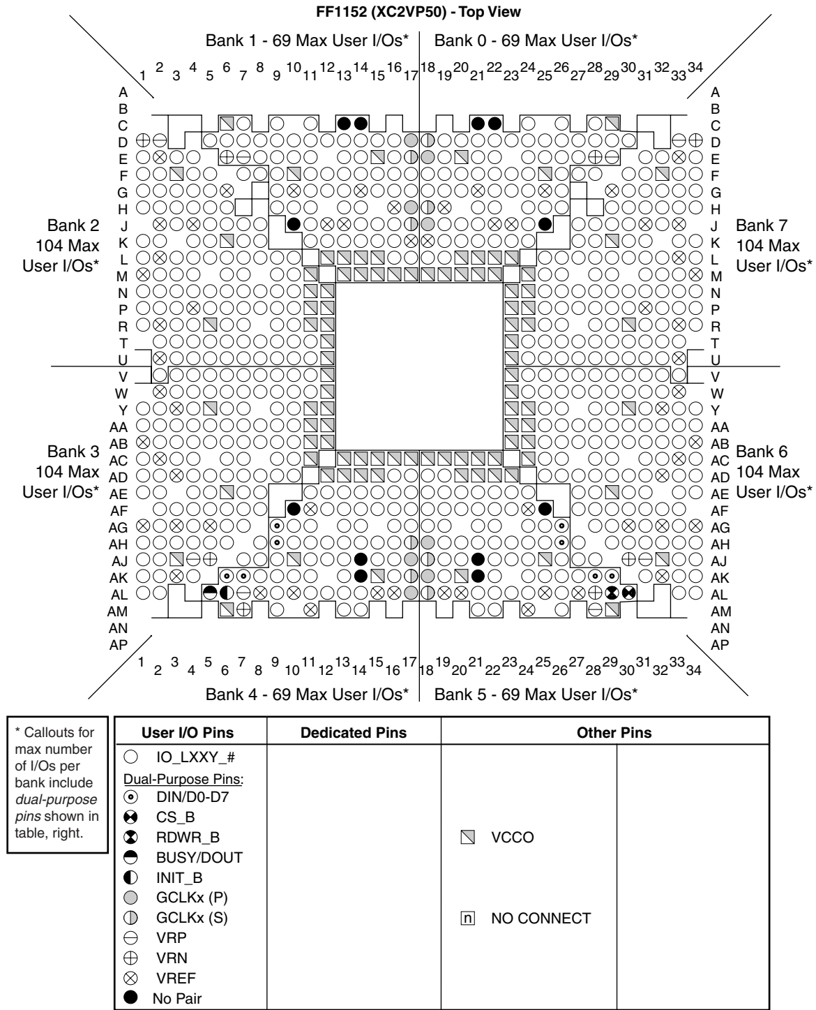
Figure 5-35: FF1152 Banked Pins (XC2VP40, XC2VP50)
