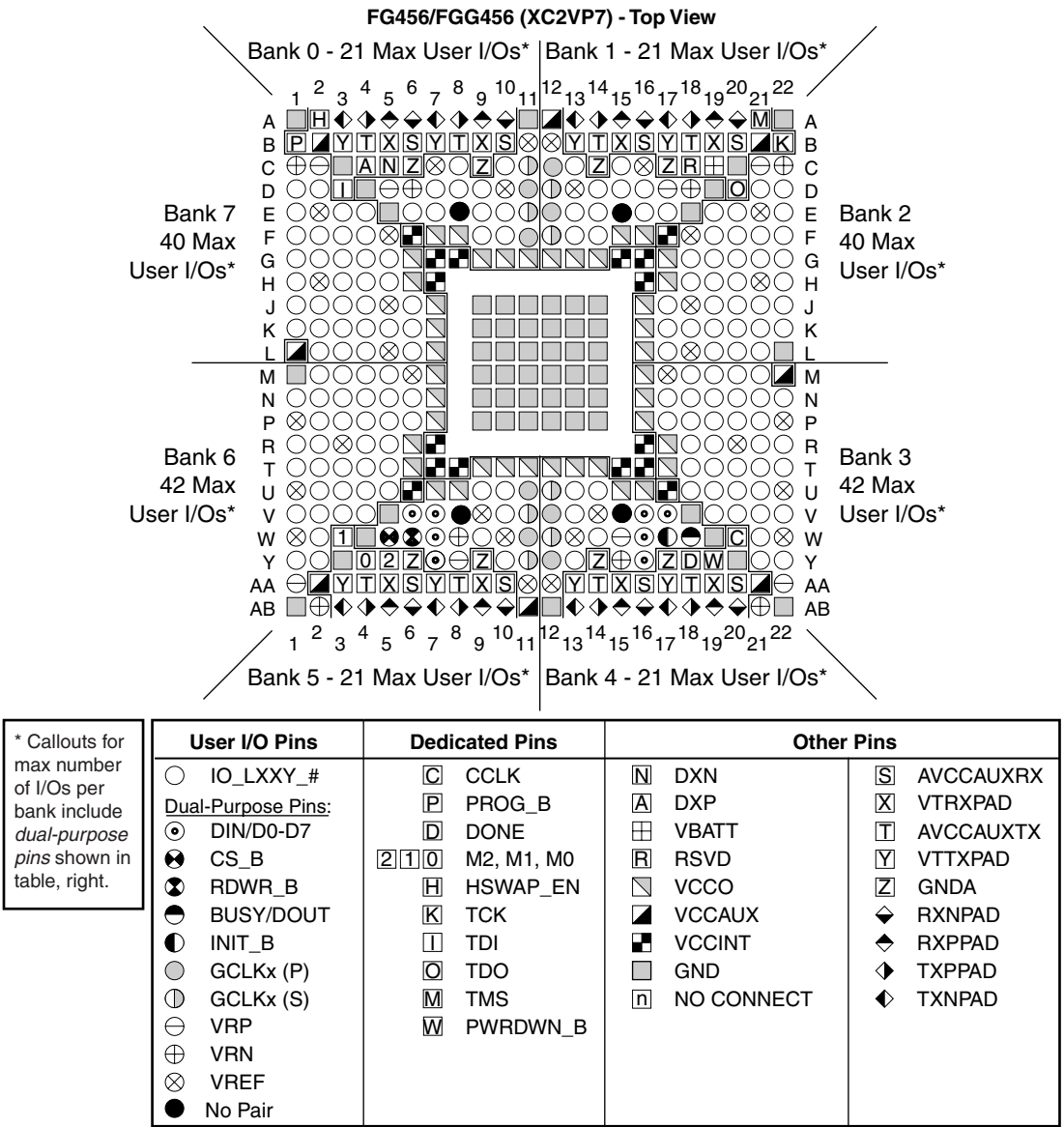
Figure 5-4: FG456/FGG456 Composite Pinout Diagram (XC2VP7)
