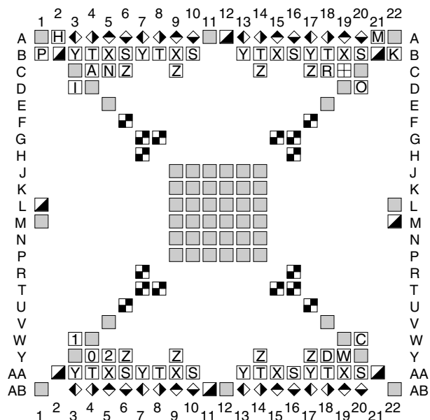
FG456/FGG456 (XC2VP7) - Top View
