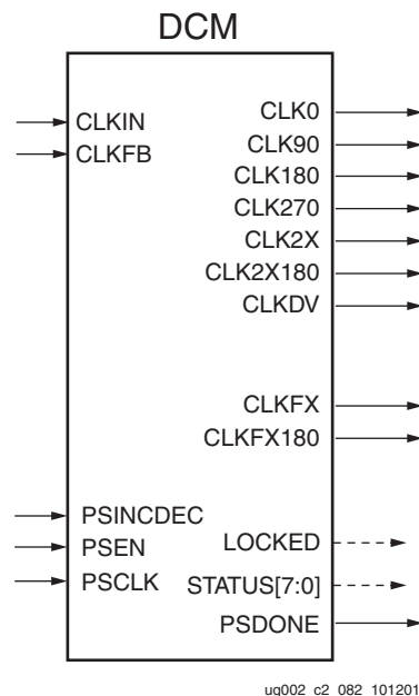
Figure 3-30: Phase Shift Outputs
