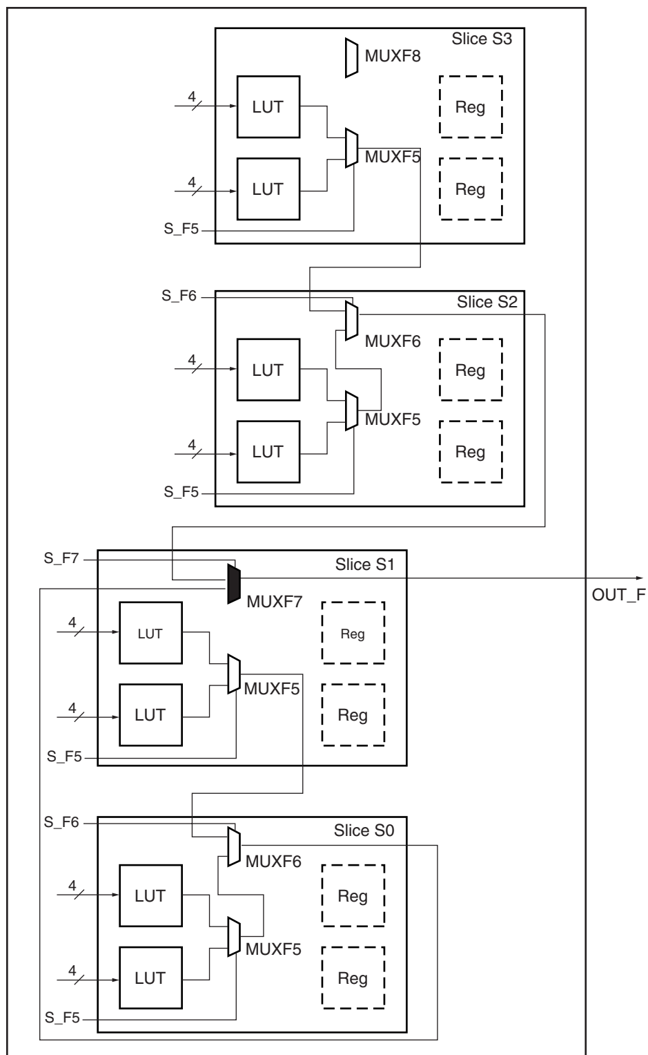
Figure 3-64: LUTs and (MUXF5, MUXF6, and MUXF7) in One CLB
