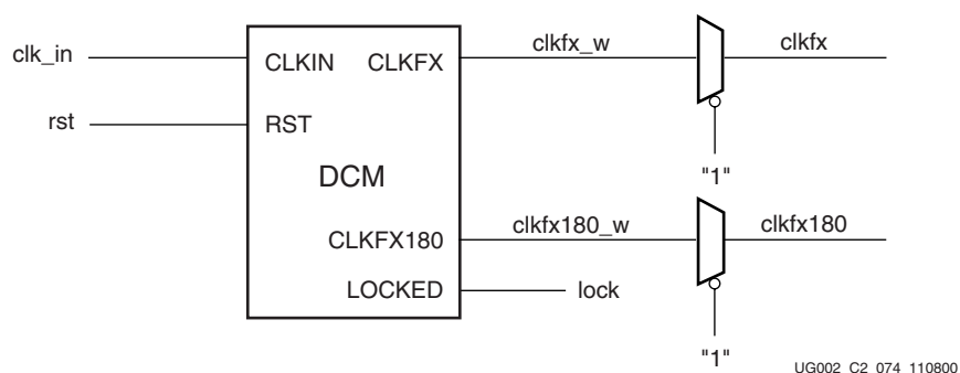
Figure 3-28: BUFG_DFS_SUBM
