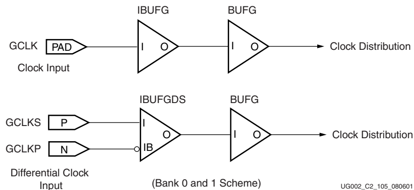
Figure 3-2: Simple Clock Distribution (Bank 0 and 1 Scheme)
