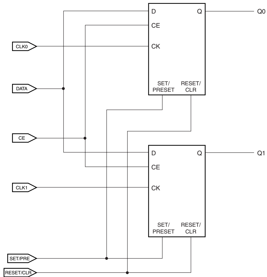
Figure 3-109: Input DDR
