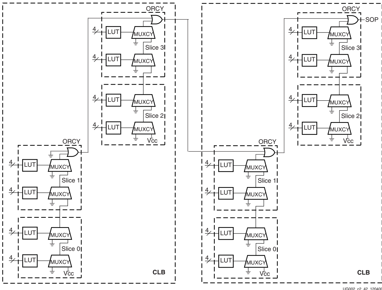
Figure 3-68: 64-bit Input SOP Design
