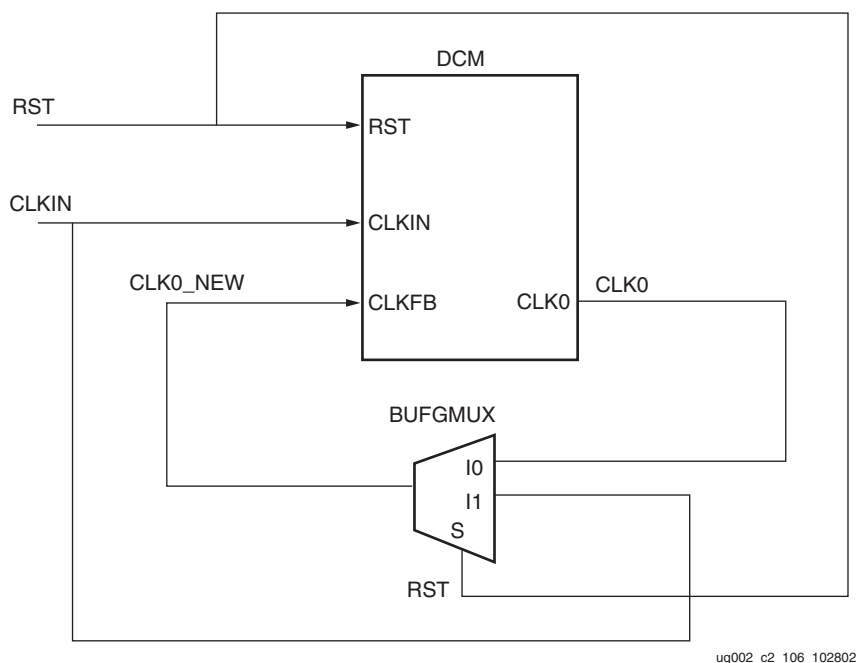
Figure 3-32: Clock Muxing for Negative PHASE_SHIFT Value
