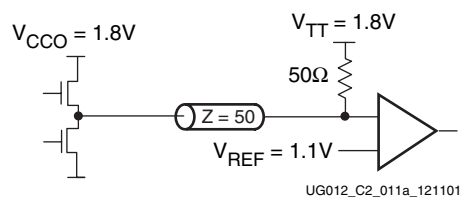
Figure 3-90: Terminated HSTL Class III (1.8V)
