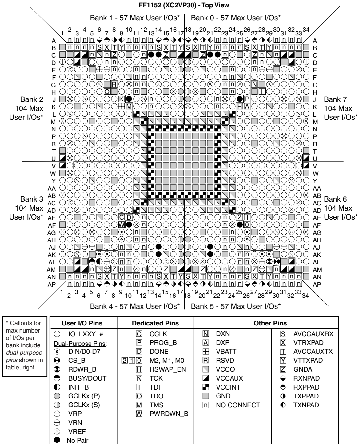
Figure 5-37: FF1152 Composite Pinout Diagram (XC2VP30)
