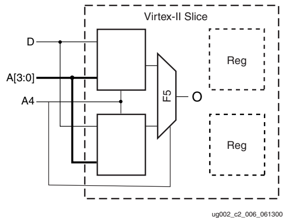
Figure 3-54: RAM32X1S Placement
