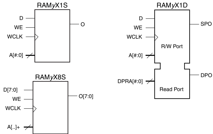
Figure 3-51: Single-Port and Dual-Port Distributed SelectRAM Primitive
