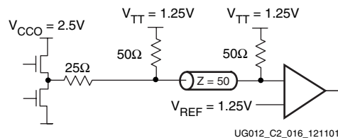
Figure 3-93: Terminated SSTL2_II
