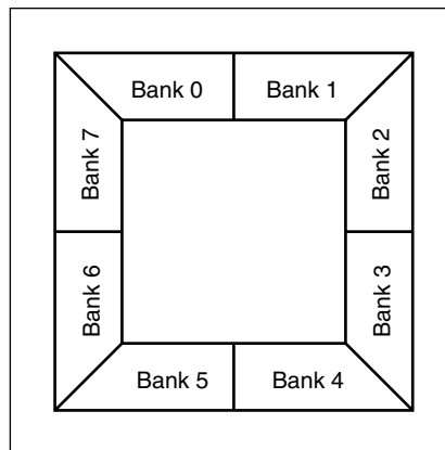
Figure 3-77: I/O Banks: Top View for Wire-Bond Package (FG)
