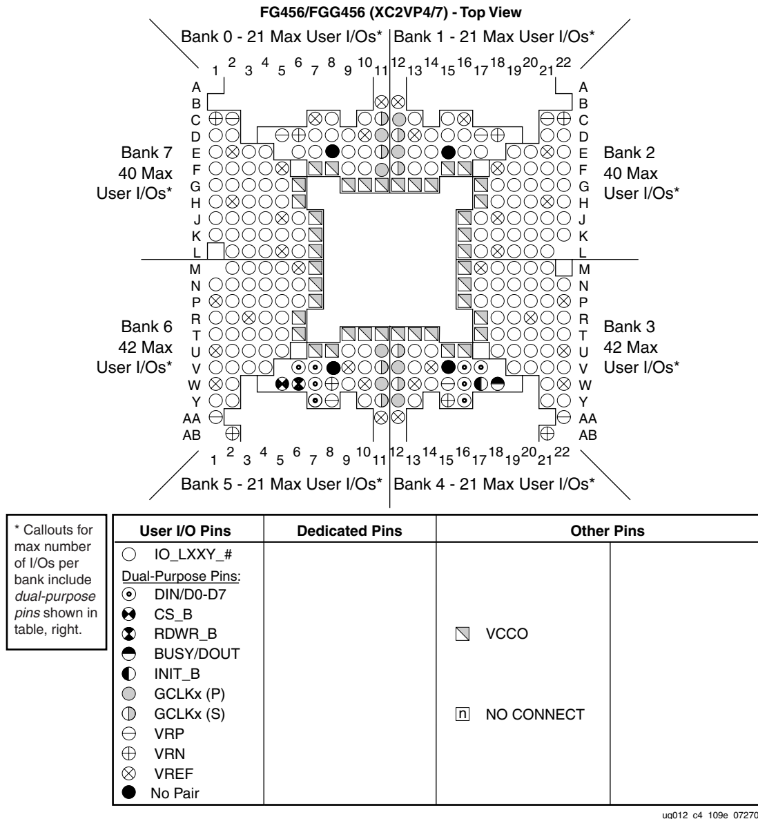
Figure 5-7: FG456/FGG456 Banked Pins (XC2VP4, XC2VP7)
