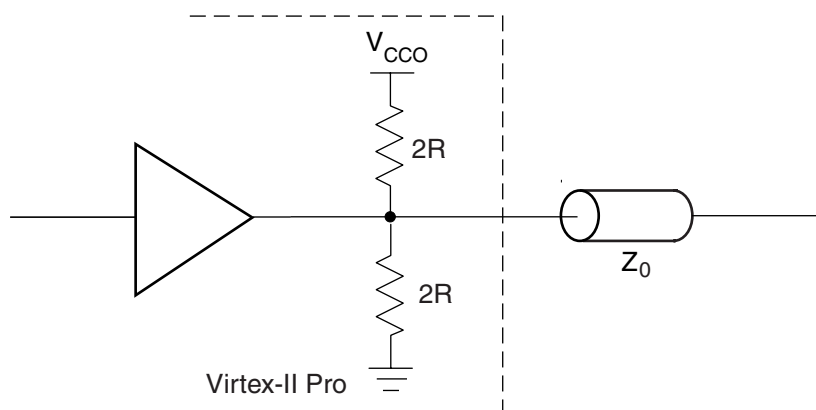
Figure 3-104: Driver with Termination to V_{CCO}/2 Using DCI Split Termination
