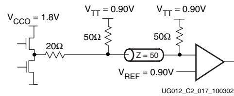
Figure 3-94: Terminated SSTL18_II
