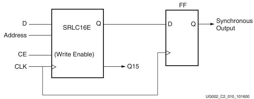
Figure 3-59: Fully Synchronous Shift Register
