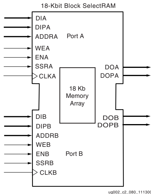
Figure 3-42: Dual-Port Data Flows
