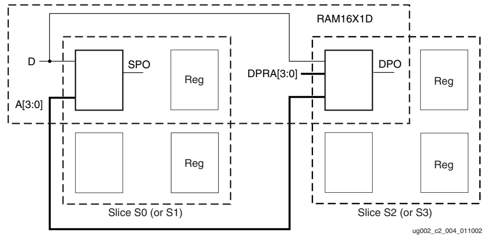
Figure 3-52: RAM16X1D Placement
