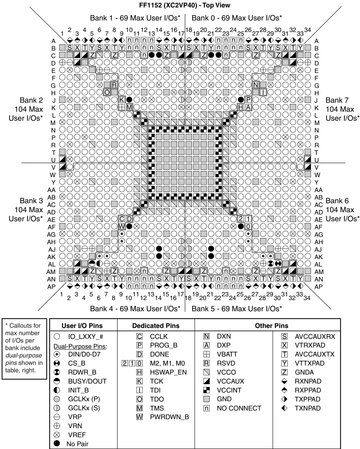
Figure 5-34: FF1152 Composite Pinout Diagram (XC2VP40)
