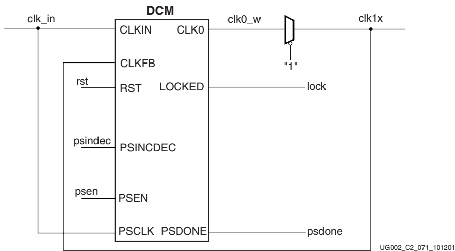
Figure 3-36: BUFG_PHASE_CLK0_SUBM
