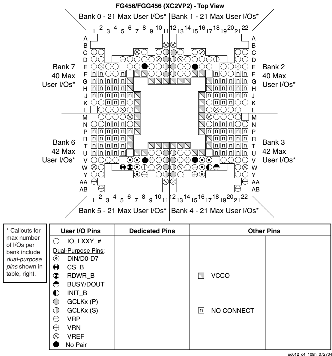
Figure 5-9: FG456/FGG456 Banked Pins (XC2VP2)
