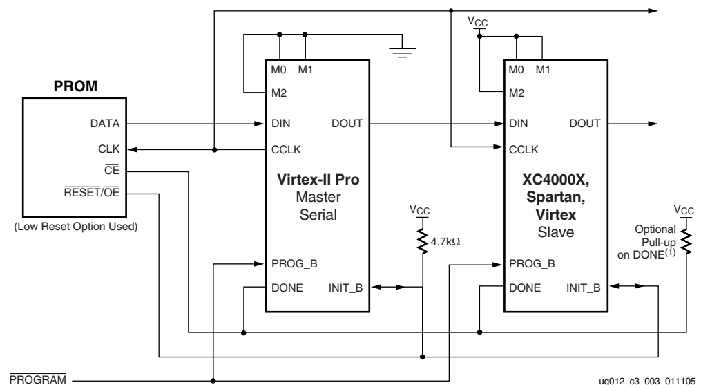
Figure 4-10: Master/Slave Serial Mode Daisy-Chain Circuit Diagram
