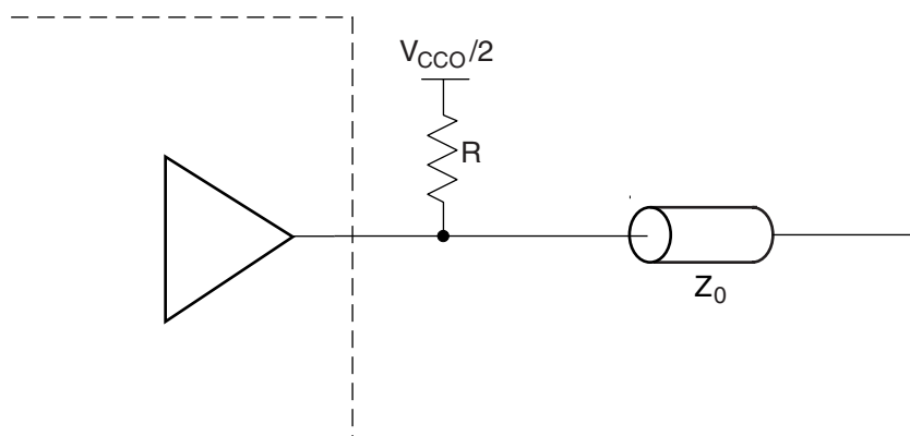
Figure 3-103: Driver with Termination to V_{CCO}/2 without DCI
