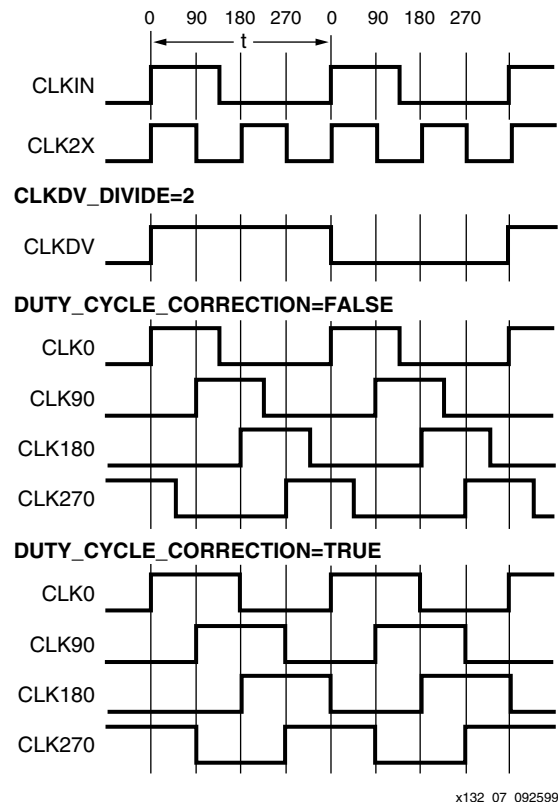
Figure 3-34: DLL Output Characteristics
