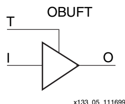
Figure 3-79: 3-State Output Buffer Symbol (OBUFT)
