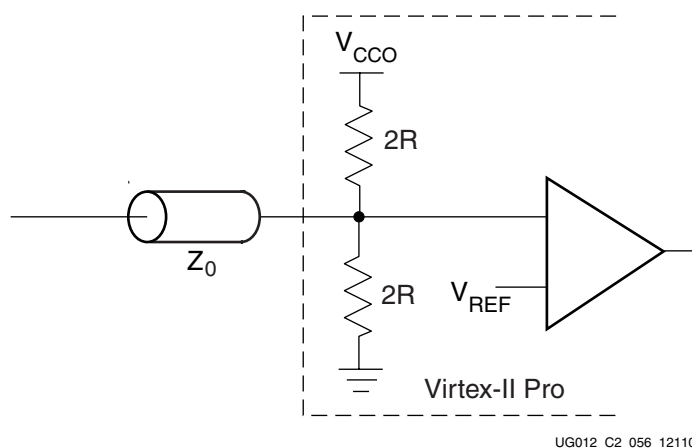
Figure 3-100: Input Termination to V_{CCO}/2 Using DCI Split Termination
