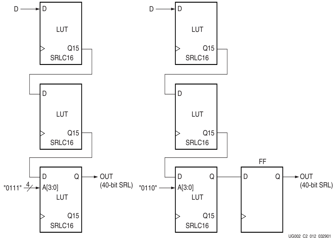
Figure 3-60: 40-bit Static-Length Shift Register
