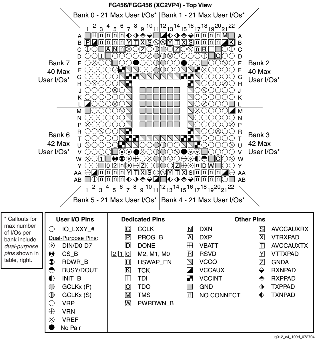
Figure 5-6: FG456/FGG456 Composite Pinout Diagram (XC2VP4)
