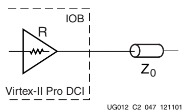
Figure 3-95: Controlled Impedance Driver
