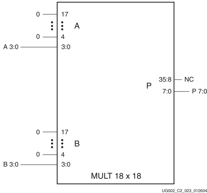
Figure 3-73: MULT4X4_U Submodule
