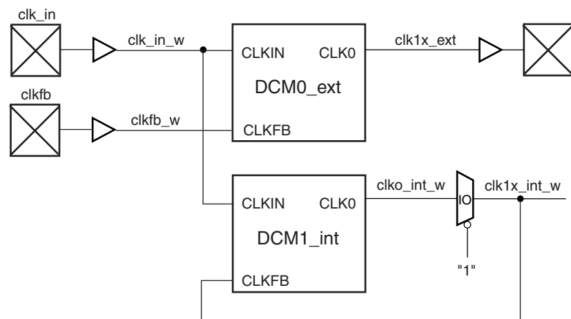
Figure 3-24: BUFG_CLK0_SUBM
