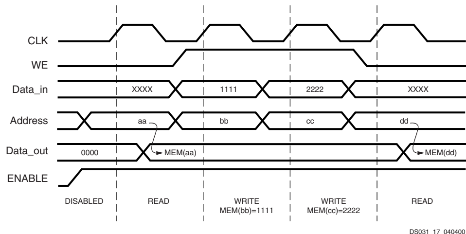
Figure 3-45: NO_CHANGE Mode Waveforms
