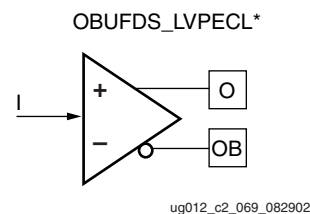
Figure 3-125: LVPECL Output Buffer Primitives
