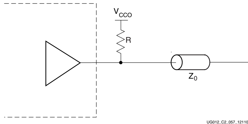
Figure 3-101: Driver with Termination to V_{CCO} without DCI
