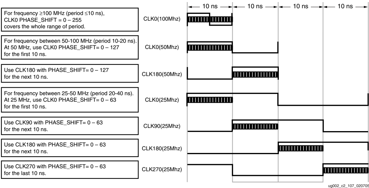
Figure 3-33: Fixed Phase Shift Example
