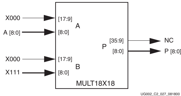
Figure 3-74: TWOS_CMP9 Submodule
