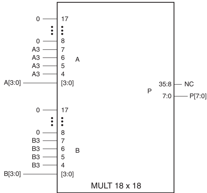
Figure 3-72: MULT4X4_S Submodule
