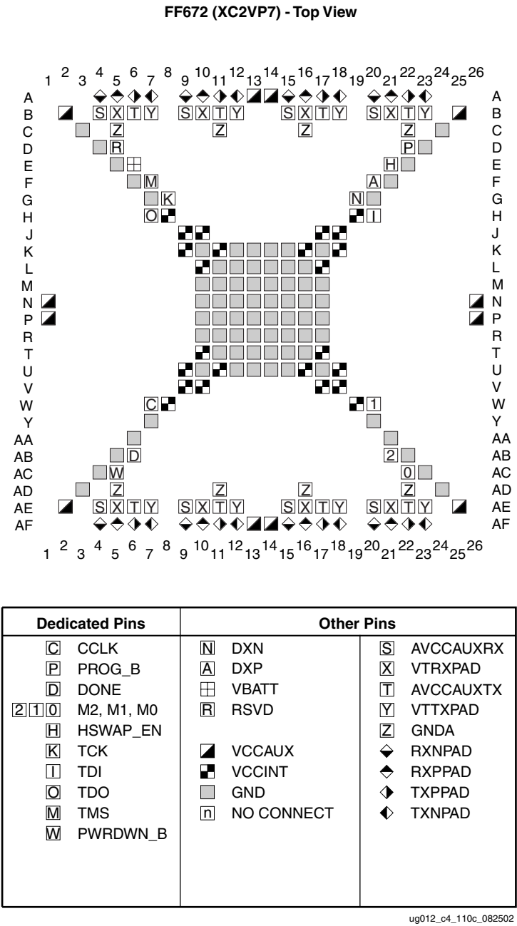
Figure 5-18: FF672 Dedicated Pins Diagram
