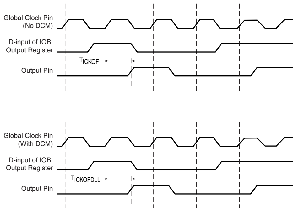
Figure 2-23: Global Clock Input to Output Timing Characteristics
