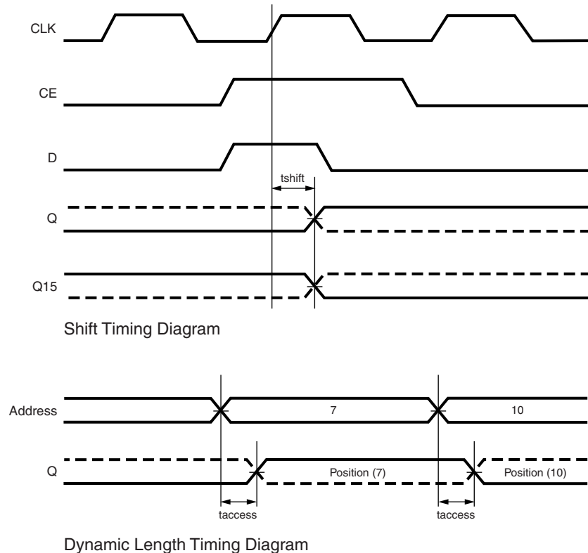
Figure 3-56: Shift- and Dynamic-Length Timing Diagrams
