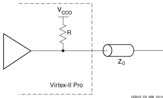
Figure 3-102: Driver with Termination to V_{CCO} Using DCI Single Termination
