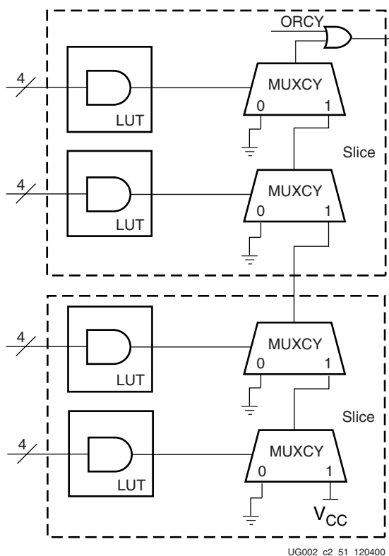
Figure 3-67: Implementing a 16-bit Wide AND Gate Using MUXCY & ORCY
