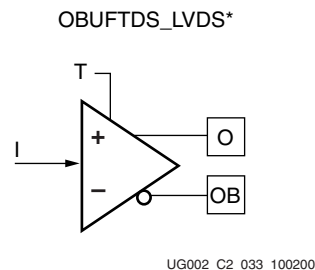
Figure 3-121: LVDS 3-State Primitives
