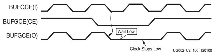
Figure 3-20: BUFGCE Waveforms
