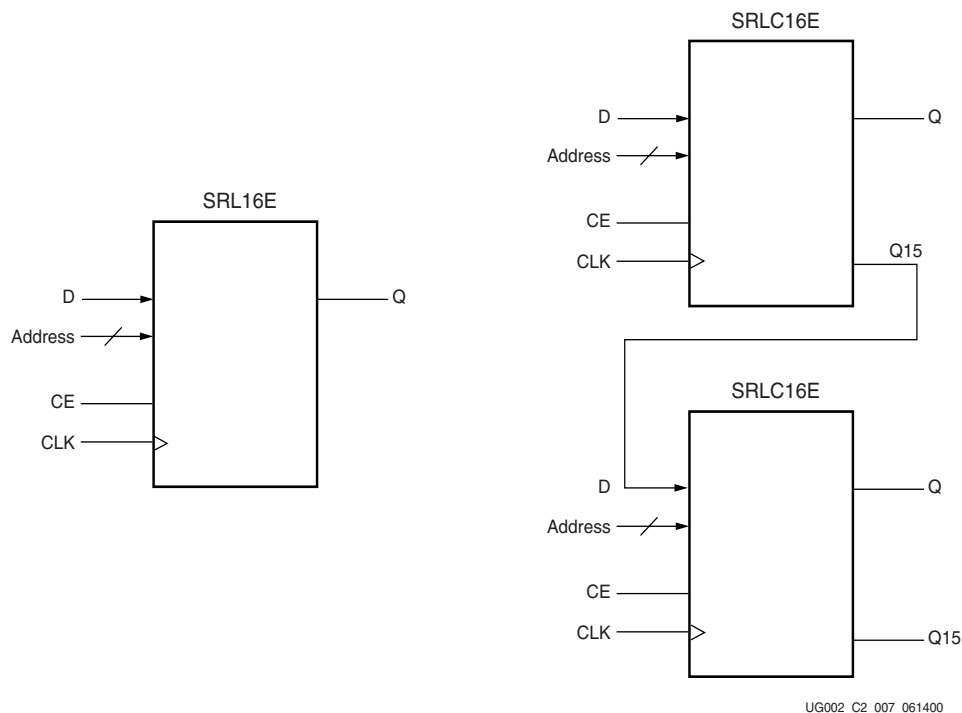
Figure 3-55: Shift Register and Cascadable Shift Register
