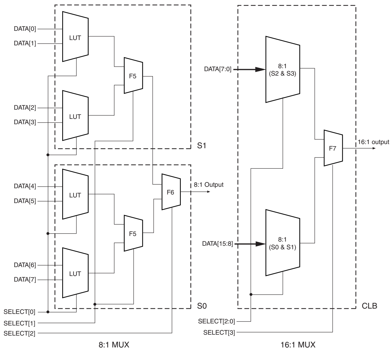
Figure 3-66: 8:1 and 16:1 Multiplexers
