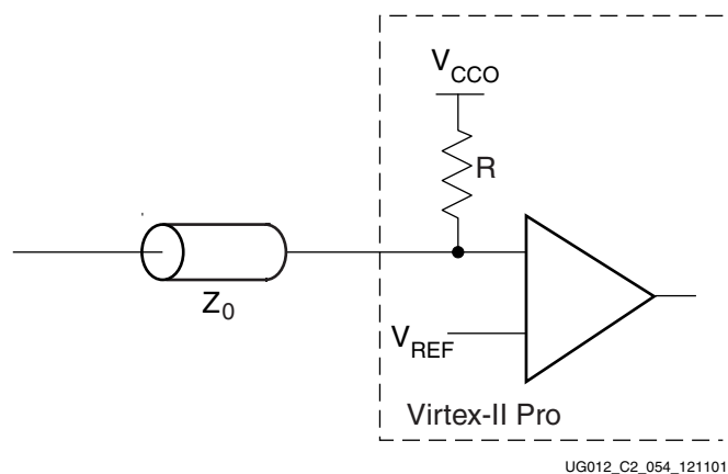
Figure 3-98: Input Termination Using DCI Single Termination
