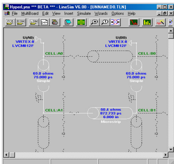
Figure 5-85: Underterminated Example
