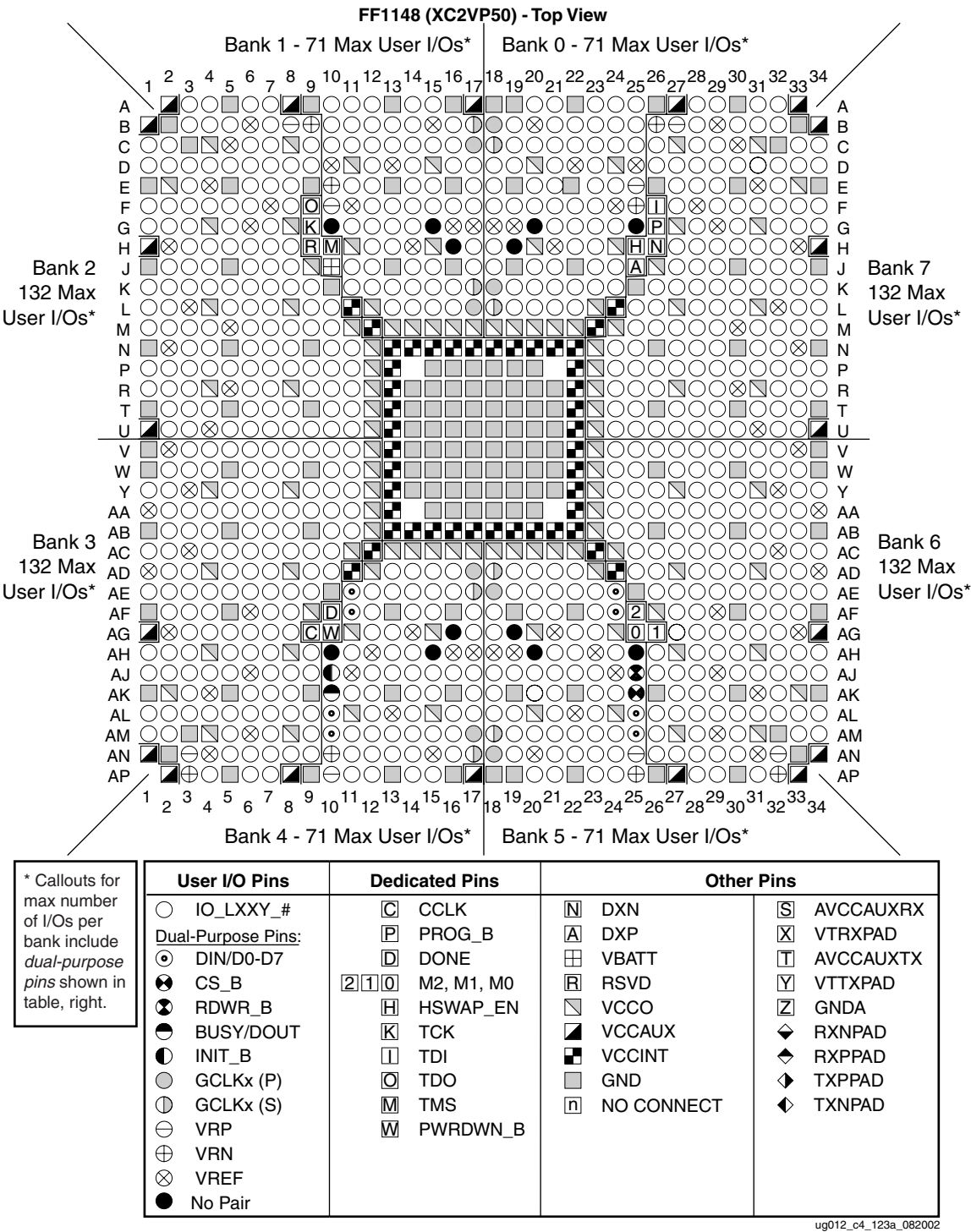
Figure 5-43: FF1148 Composite Pinout Diagram (XC2VP50)
