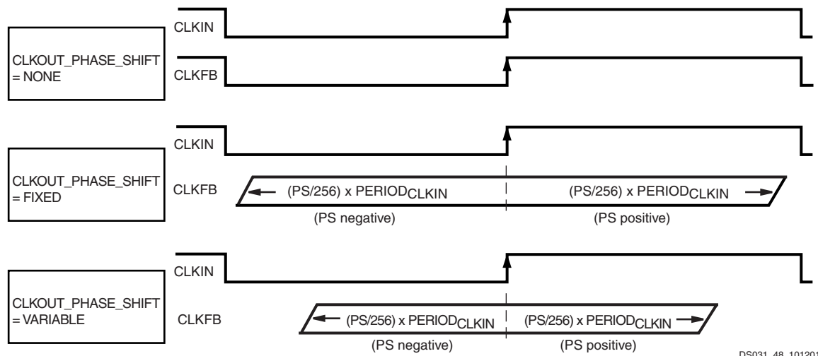
Figure 3-31: Phase Shift Effects
