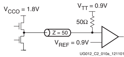
Figure 3-88: Terminated HSTL Class I (1.8V)
