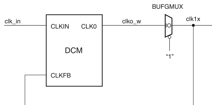
Figure 3-24: BUFG_CLK0_SUBM
