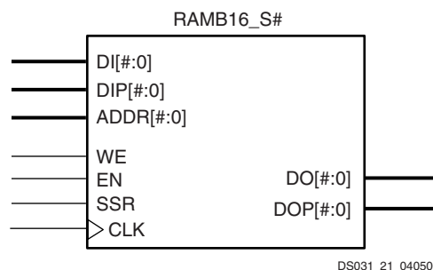
Figure 3-48: Single-Port Block RAM Primitive
