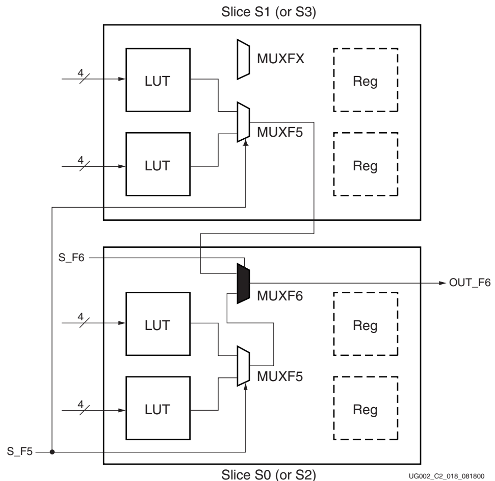
Figure 3-63: LUTs and (MUXF5 and MUXF6) in Two Slices
