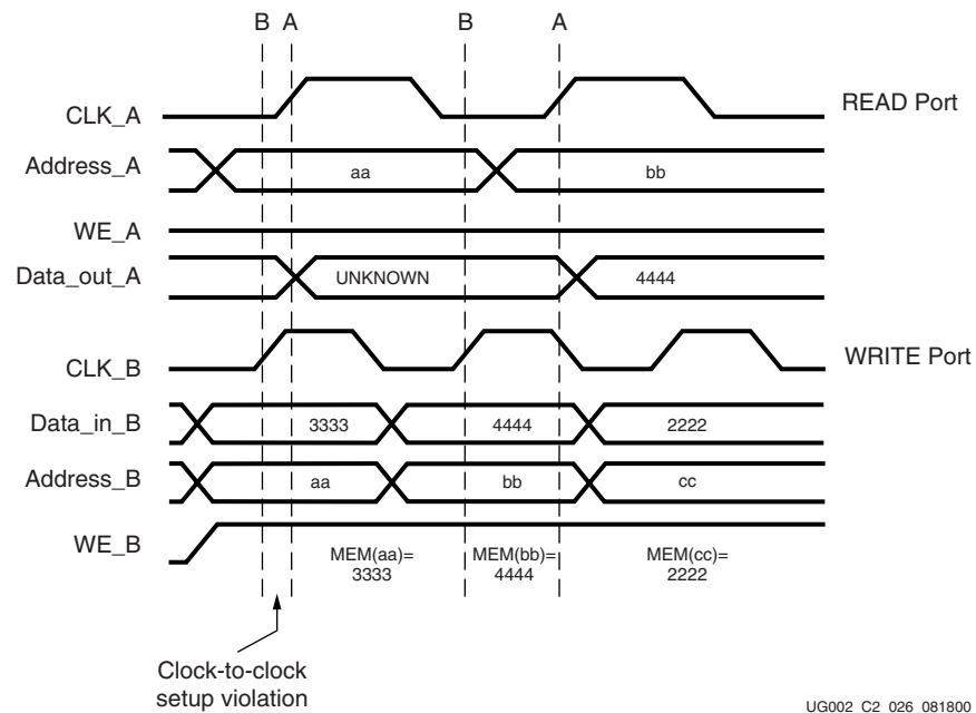
Figure 3-46: READ-WRITE Conditions
