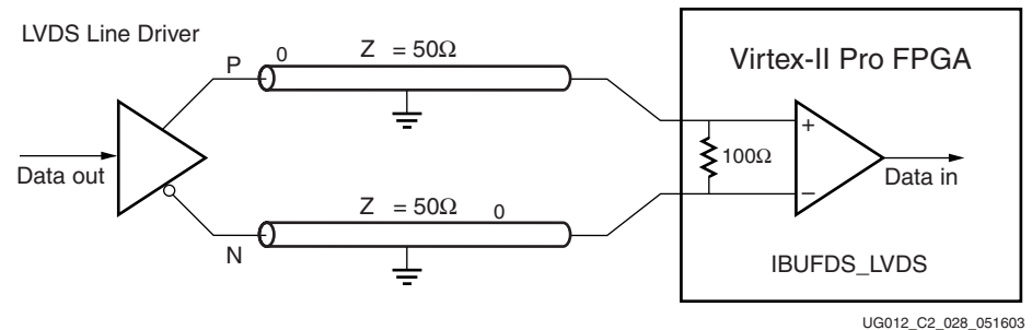
Figure 3-118: LVDS Receiver Termination
