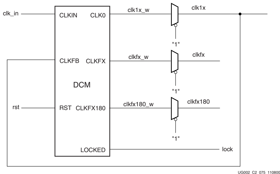
Figure 3-29: BUFG_DFS_FB_SUBM
