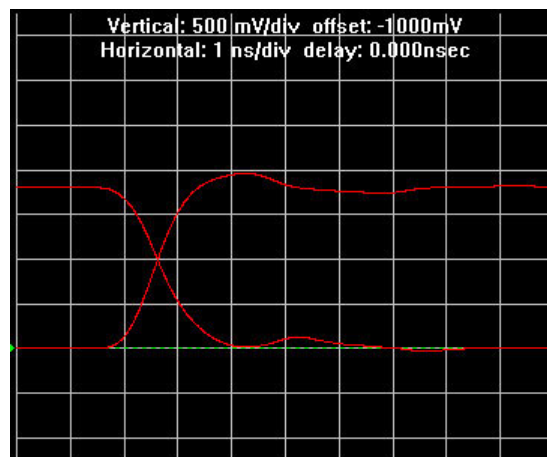
Figure 5-87: DCI Driver Example
