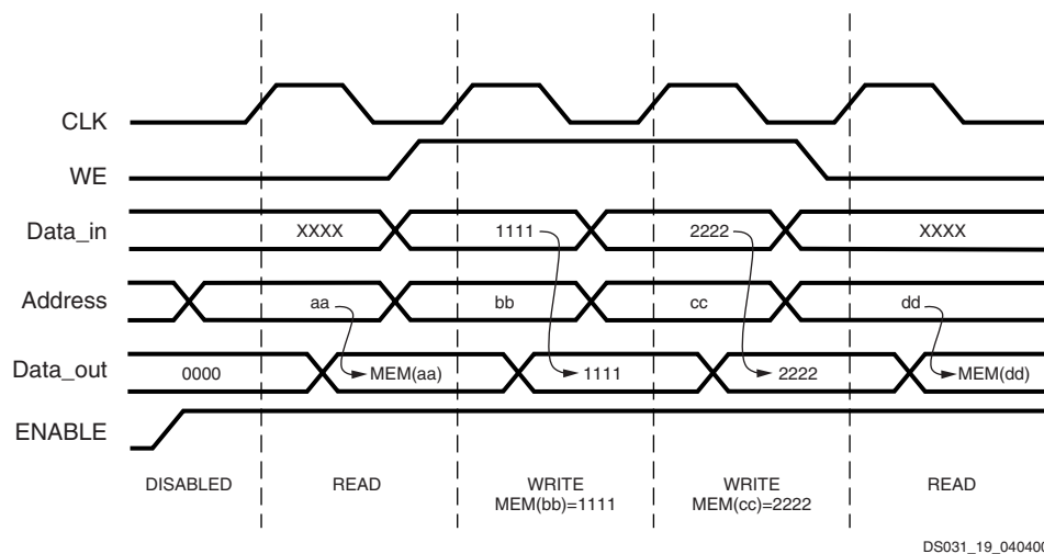
Figure 3-43: WRITE_FIRST Mode Waveforms
