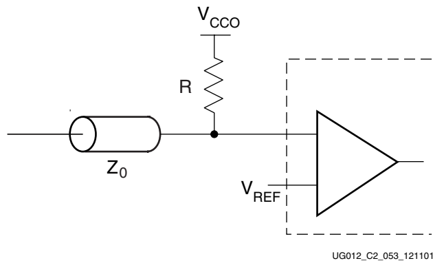
Figure 3-97: Input Termination to V_{CCO} without DCI
