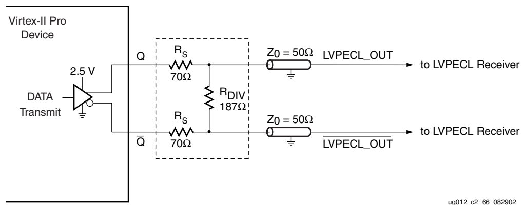
Figure 3-126: LVPECL Transmitter Termination
