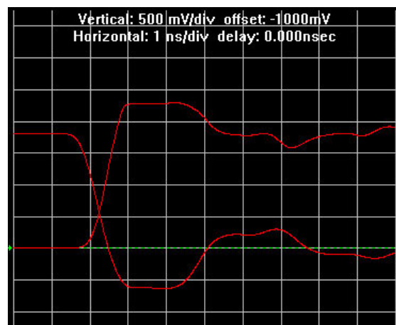
Figure 5-85: Underterminated Example
