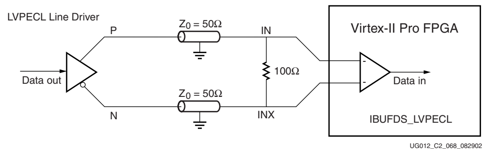
Figure 3-124: LVPECL Receiver Termination
