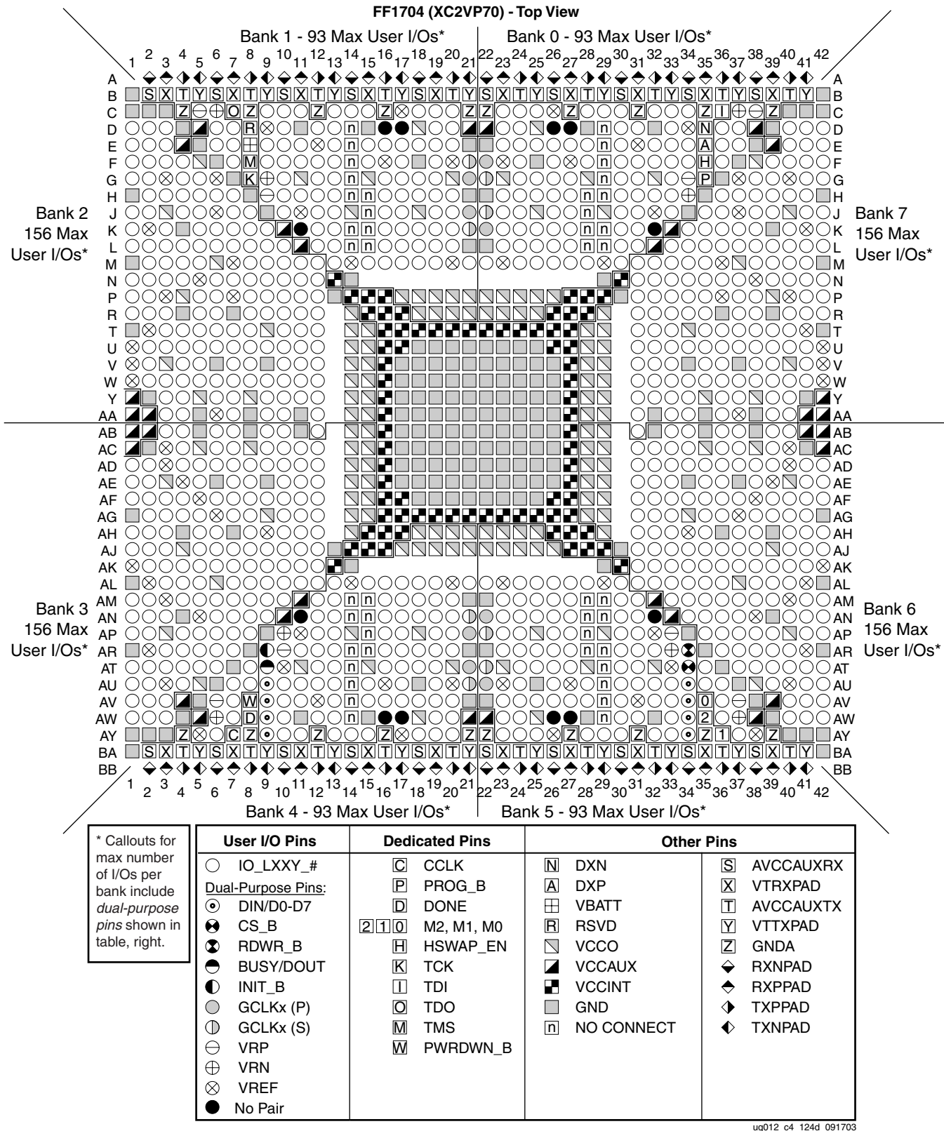
Figure 5-55: FF1704 Composite Pinout Diagram (XC2VP70)
