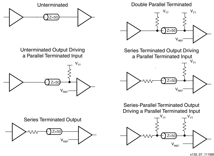
Figure 3-81: Overview of Standard Input and Output Termination Methods
