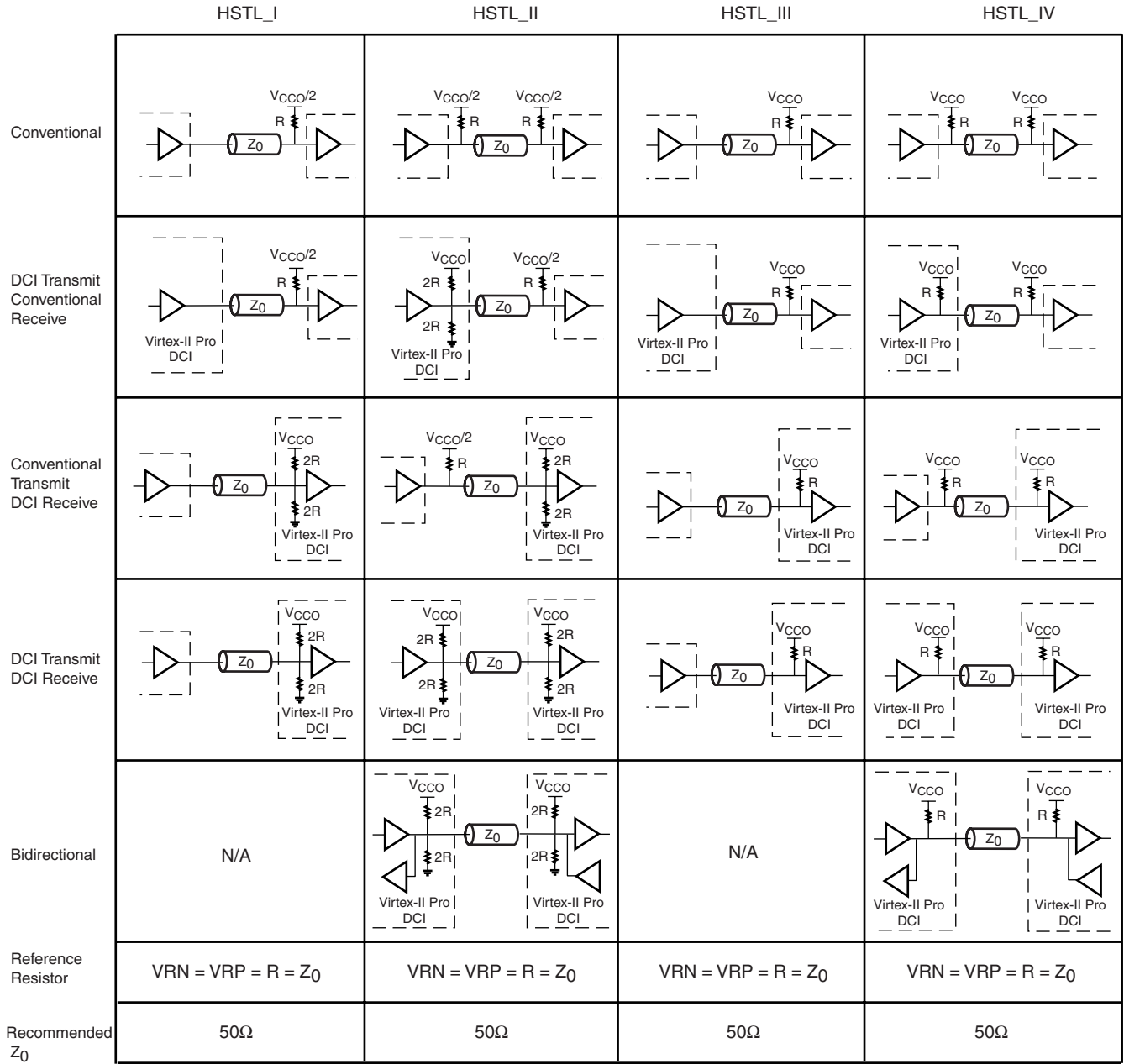
Figure 3-105: HSTL DCI Usage Examples
