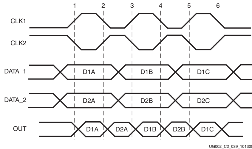
Figure 3-112: Output DDR Timing Diagram
