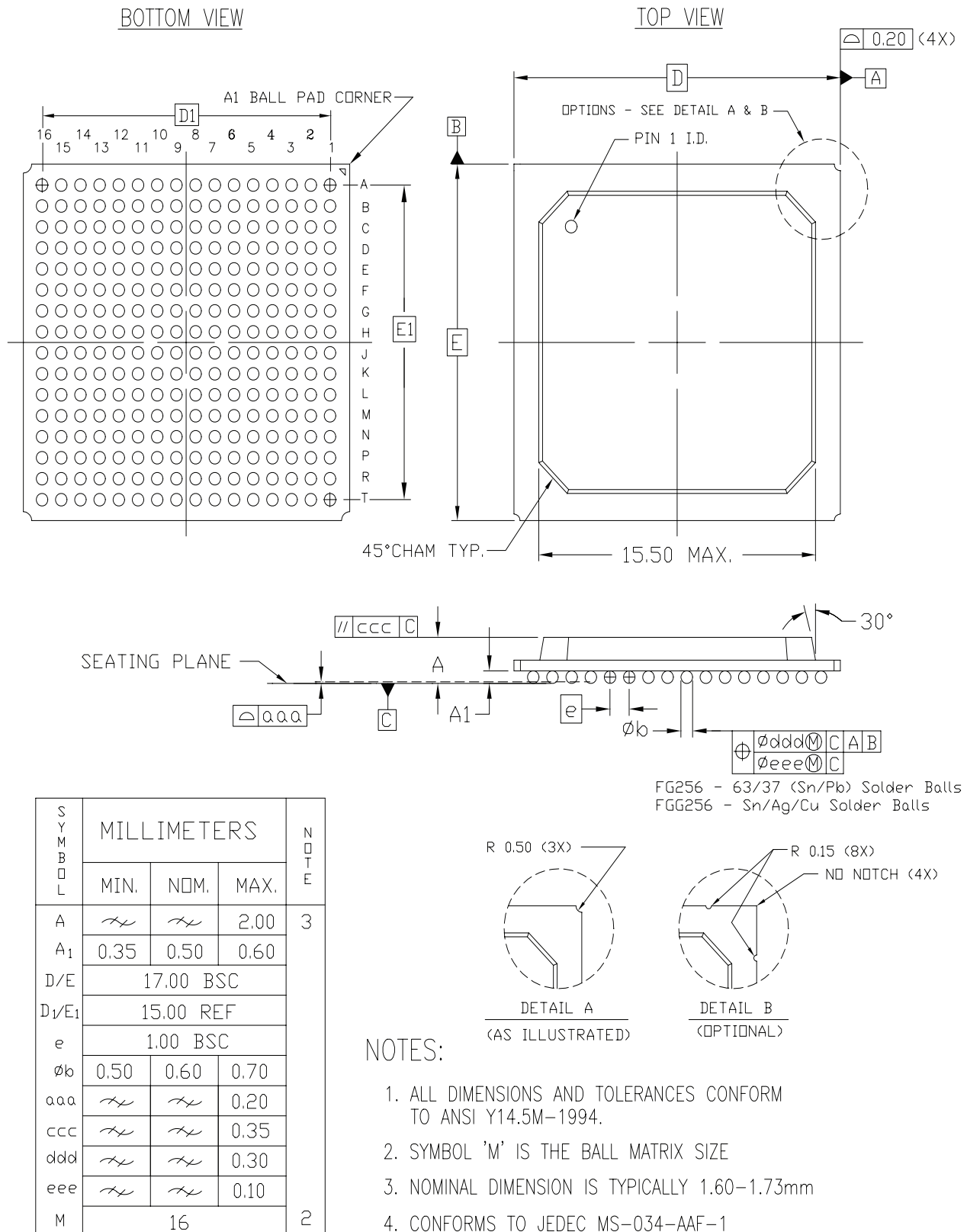
Figure 5-64: FG256/FGG256 Fine-Pitch BGA Package
