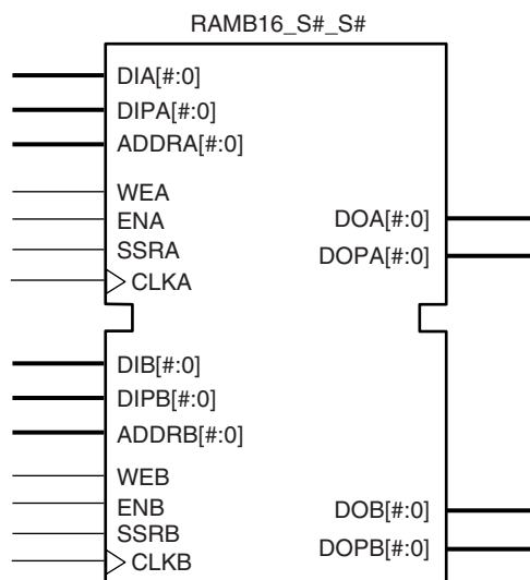
Figure 3-47: Dual-Port Block RAM Primitive
