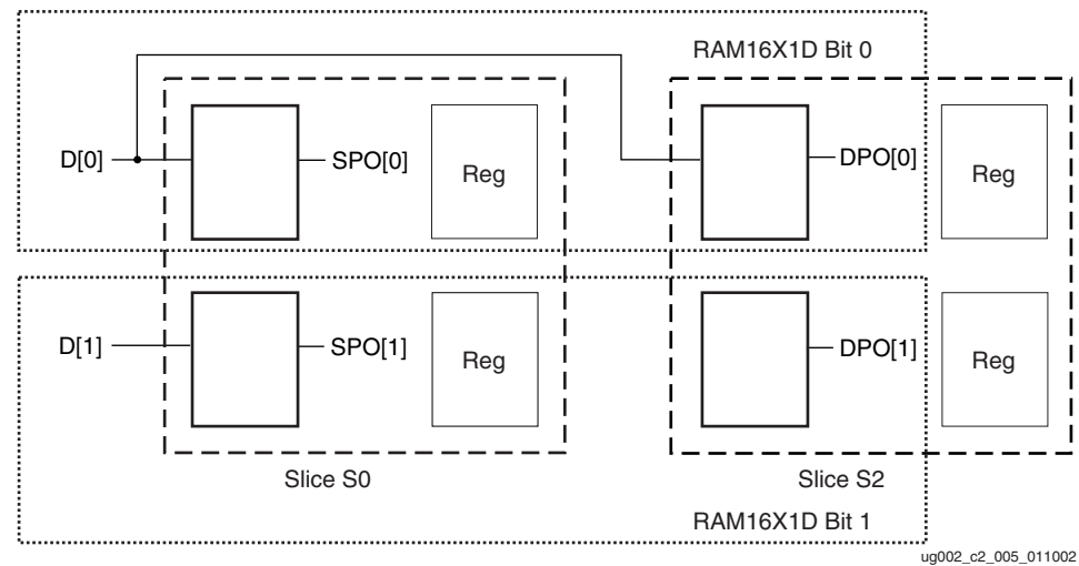
Figure 3-53: Two RAM16X1D Placement
