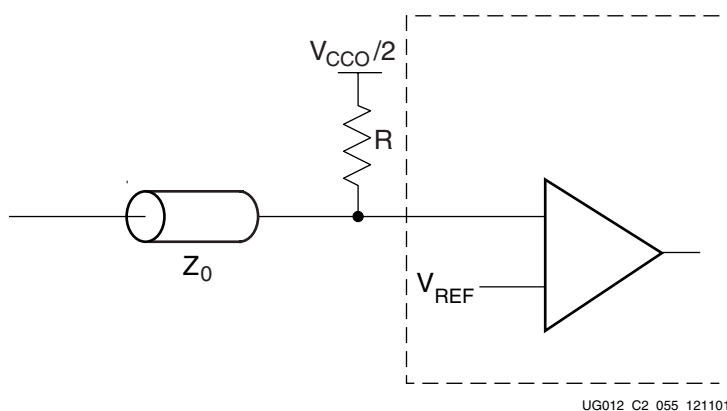
Figure 3-99: Input Termination to V_{CCO}/2 without DCI
