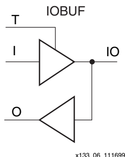
Figure 3-80: Input/Output Buffer Symbol (IOBUF)
