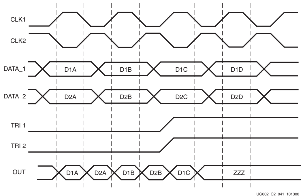
Figure 3-114: Timing Diagram for Output DDR With 3-State Control
