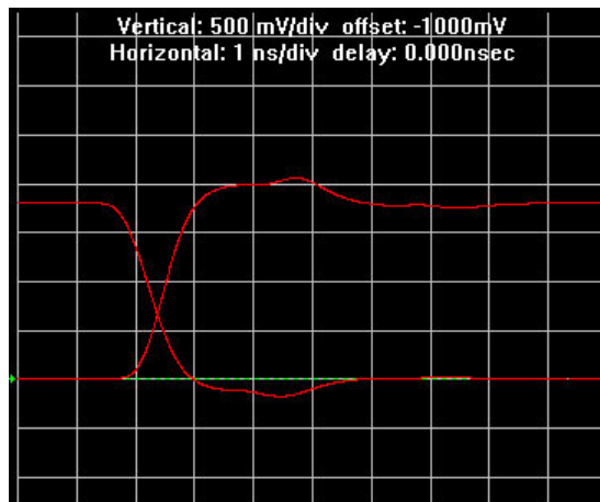
Figure 5-86: Series Termination Example
