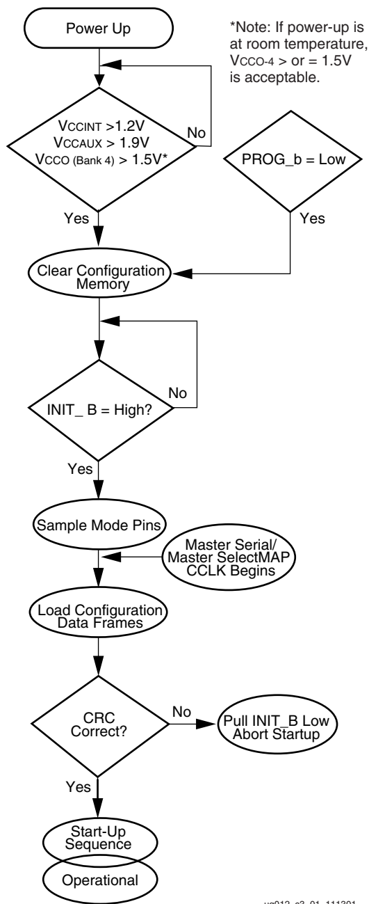
Figure 4-1: Configuration Process
