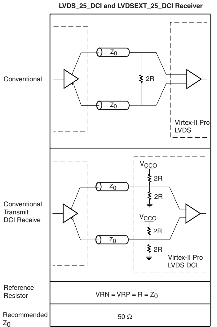
Figure 3-107: LVDS DCI Usage Examples
