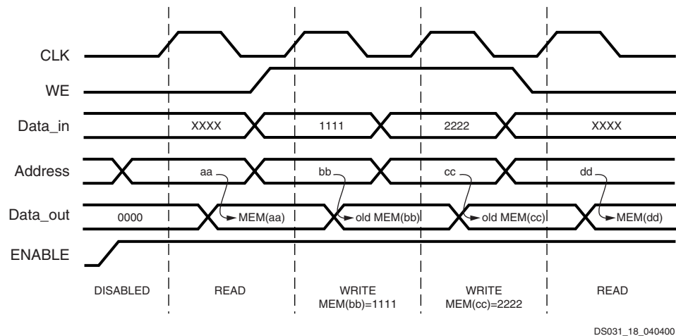
Figure 3-44: READ_FIRST Mode Waveforms
