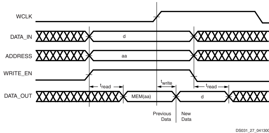
Figure 3-50: Write Timing Diagram
