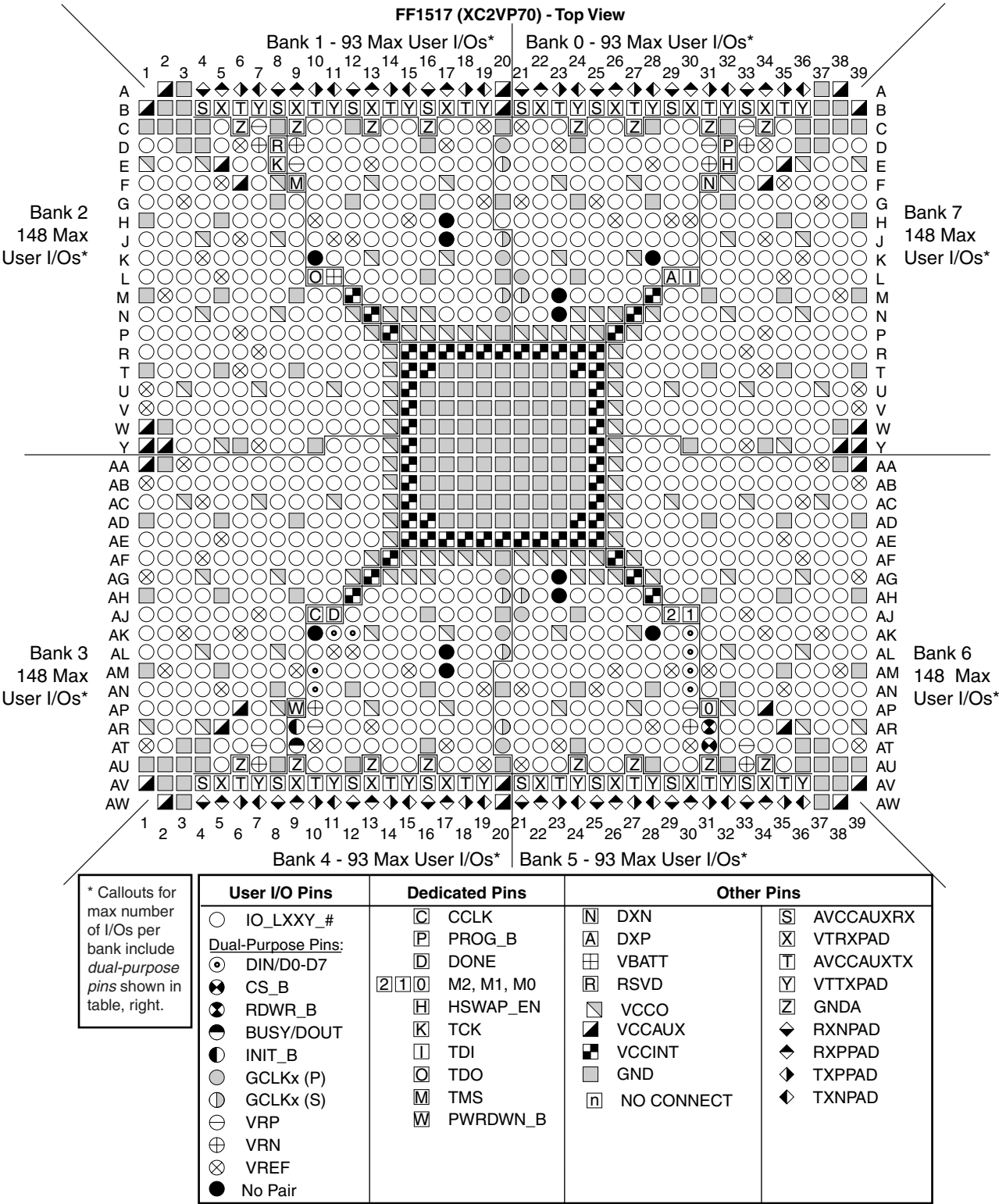
Figure 5-48: FF1517 Composite Pinout Diagram (XC2VP70)
