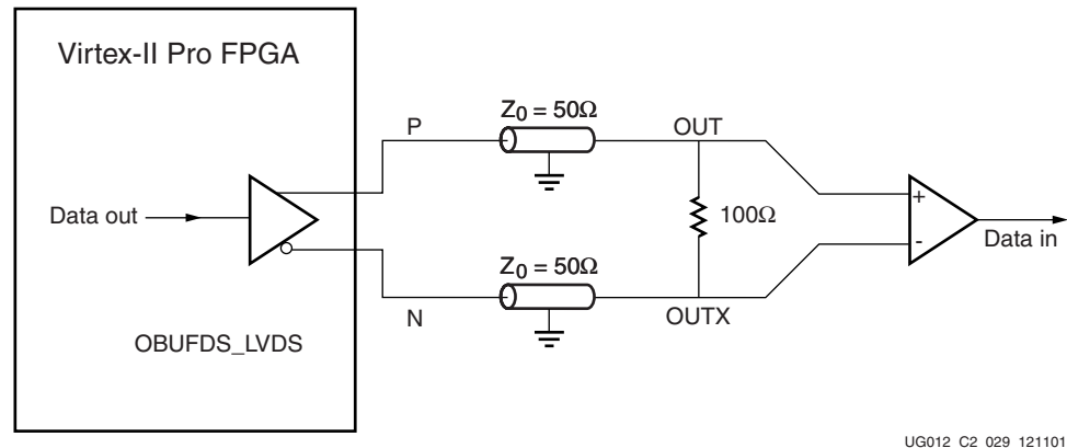
Figure 3-120: LVDS Transmitter Termination
