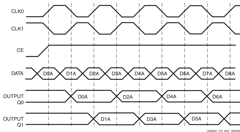
Figure 3-110: Input DDR Timing Diagram
