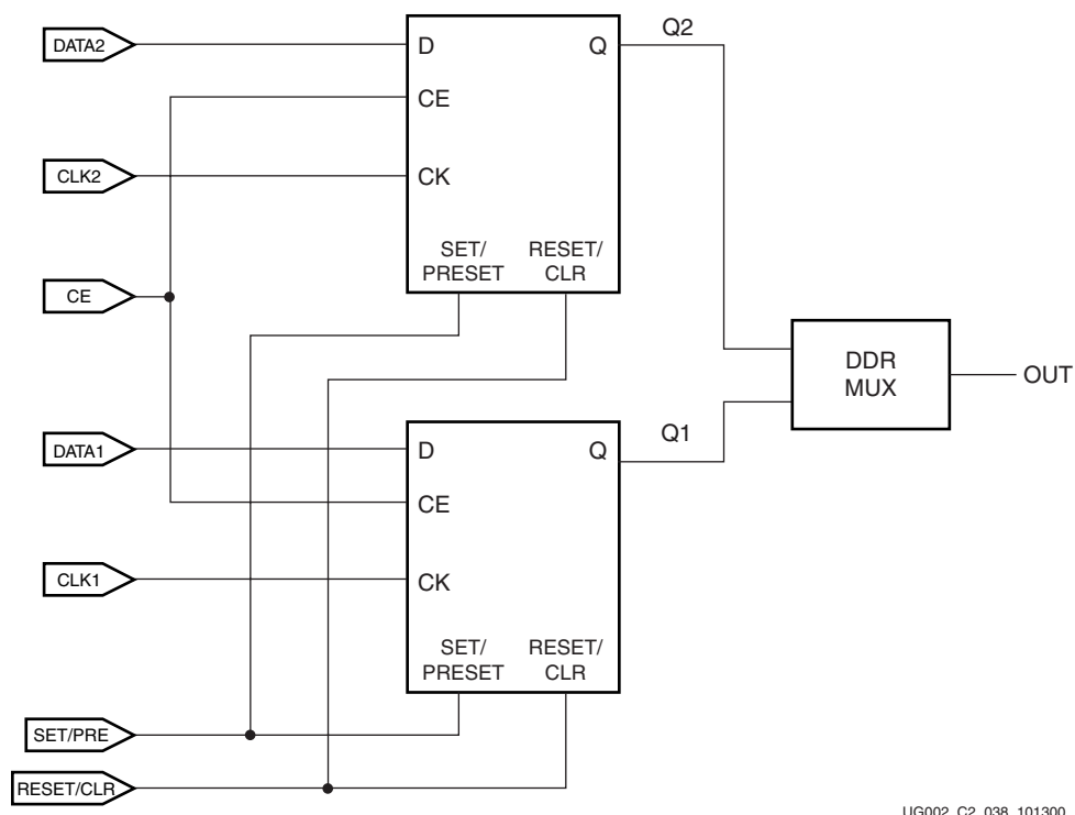
Figure 3-111: Output DDR
