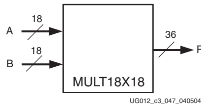
Figure 3-69: Embedded Multiplier
