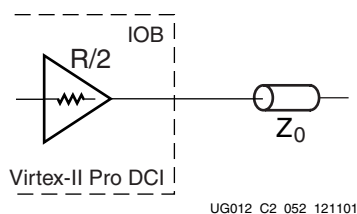
Figure 3-96: Controlled Impedance Driver with Half Impedance
