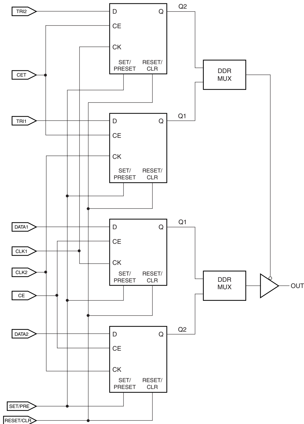
Figure 3-113: Output DDR With 3-State Control
