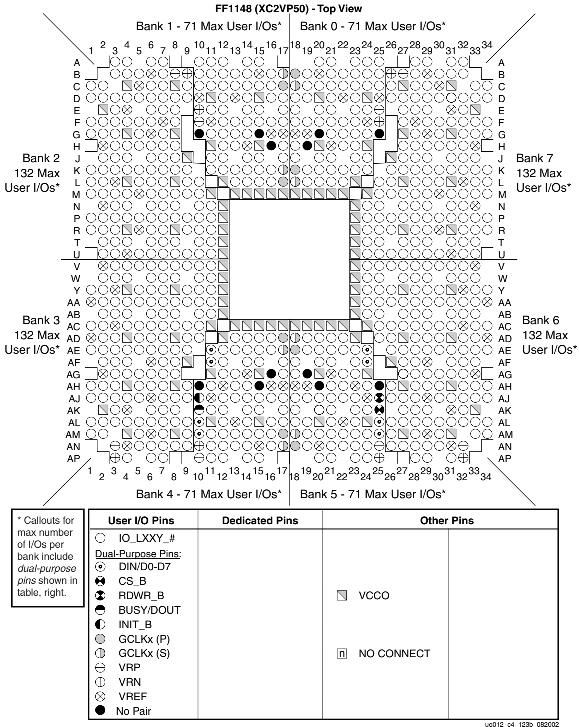
Figure 5-44: FF1148 Banked Pins (XC2VP50)
