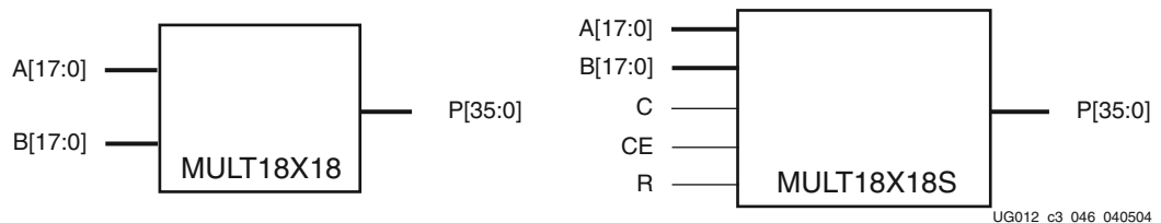
Figure 3-70: Combinatorial and Registered Multiplier Primitives
