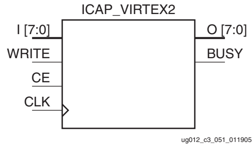
Figure 4-21: ICAP_VIRTEX2 Primitive
