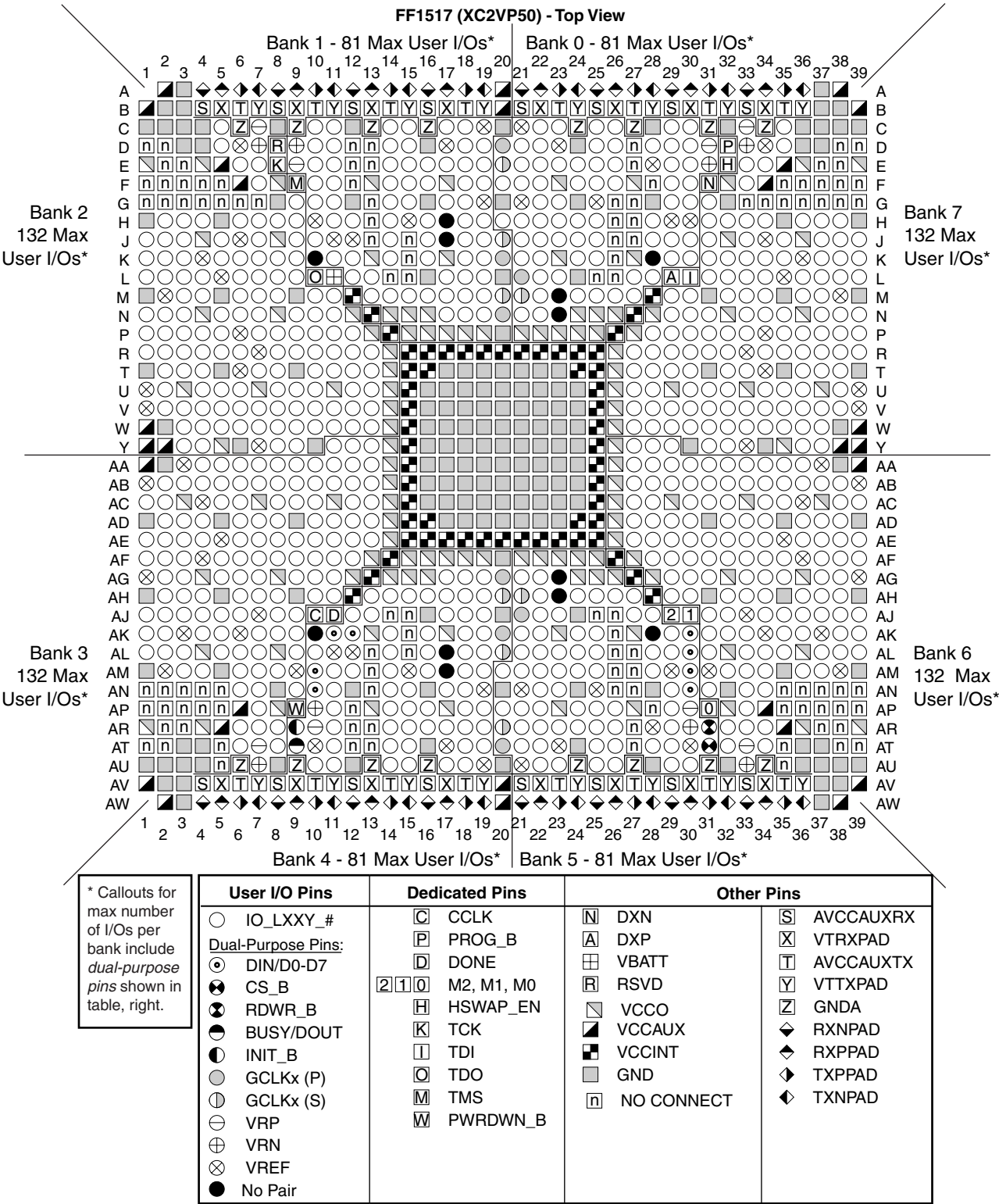
Figure 5-50: FF1517 Composite Pinout Diagram (XC2VP50)
