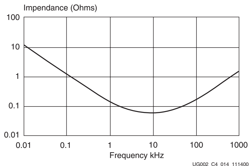
Figure 5-74: 1500 \mu\text{F} Electrolytic Capacitor Frequency Response Curve
