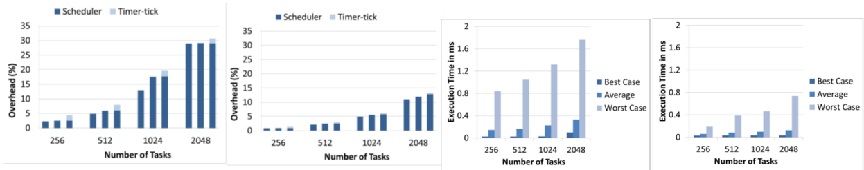
(b) Performance of a software implemented EDF scheduler compared to one based on SW/HW co-designed priority queue.
