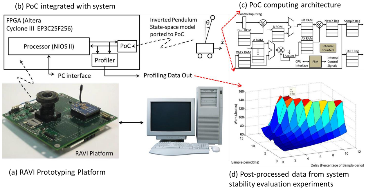
Figure 5: (a) RAVI FPGA-based prototyping platform, (b) PoC substituted for an inverted pendulum plant for evaluating system stability for variation in controller response time, (c) hardware computing architecture of the PoC, (d) example post-processed data showing actuator effort vs. sensors sample period and controller computation delay.
