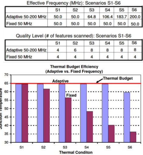
Figure 10: a) Run-time parameterizable FPGA-based image processing application, where application clock frequency, and number of Masks applied to an image (i.e. features scanned for) adjust to maximize performance for a given “Thermal Budget”, b) Summary of experimental results that quantify performance improvement when using temperature feedback to dynamically adjust application parameters, as compared to a static design that must meet thermal constraints under worst-case operating conditions. Scenario S1 represents worst-case operation conditions (e.g. broken fan, high ambient temperature), while S6 represents best-case operating conditions (e.g. operational fans, and low ambient temperature) [19].
