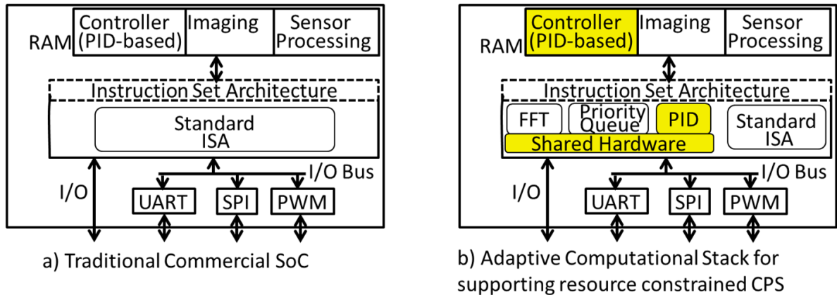
Figure 3: Vision for hardware architectural support of resource constrained CPS (Cyber Physical Systems)
