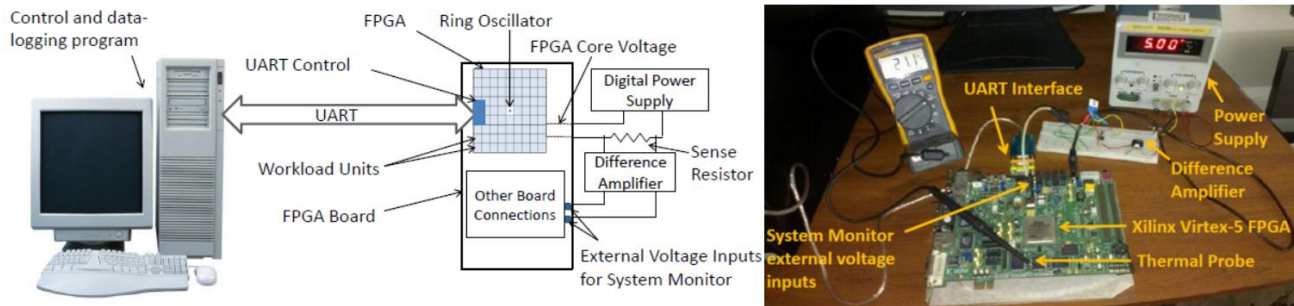
Figure 8: Experimentation setup for monitoring FPGA current draw to track workload intensity
