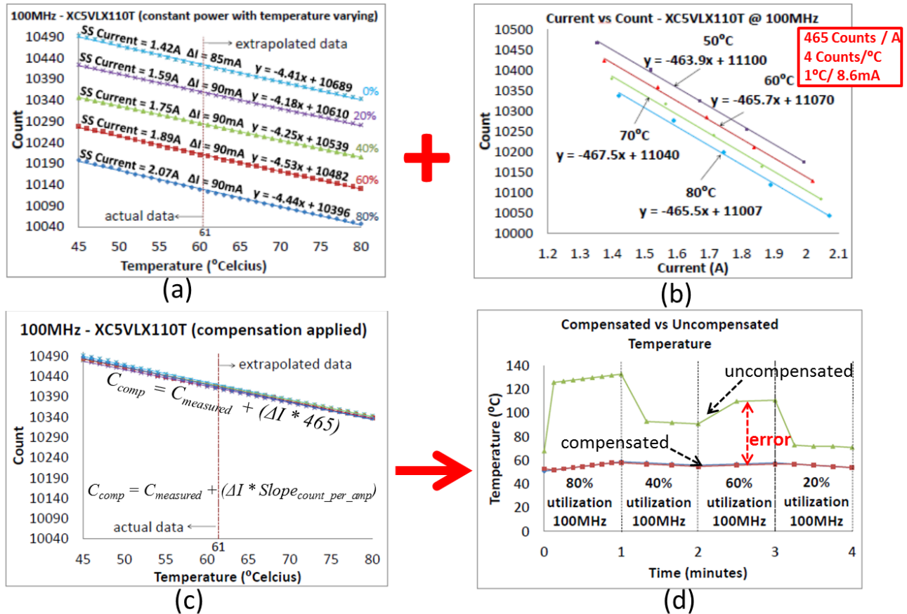
Figure 9: a) Observation that ring oscillator frequency vs. temperature relation varies with the workload intensity of the FPGA (0% - 80% utilization), b) results of experiments to characterize FPGA current draw vs. ring oscillator frequency for lines of constant temperature, c) the application of the results of characterization experiments to (a) to compensate for non-thermal effects of workload intensity on ring oscillator frequency, d) experimental evaluation of compensation technique, as can be seen the error between the compensated ring-oscillator thermometer and actual temperature is not noticeable compared to the uncompensated ring-oscillator thermometer as workload intensity is varied. .
