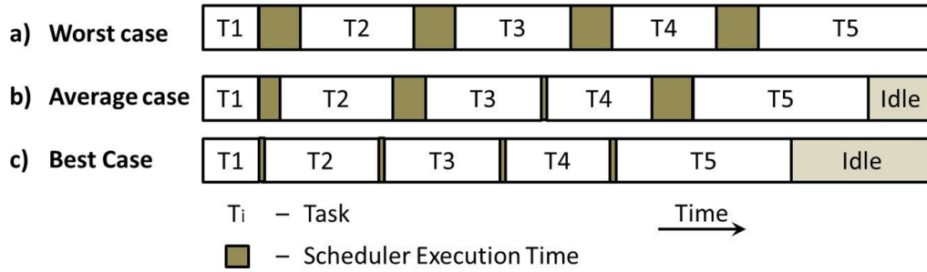
Figure 6: In order to allow analytical analysis of schedule feasibility, worst-case execution time (WCET) typically needs to be assumed. Thus, scheduler execution time variations that cause large differences between WCET and typical case execution time reduce utilization of system computing resources.
