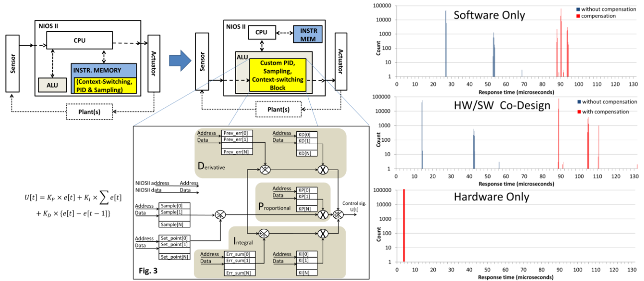
Figure 4: a) FPGA-based evaluation setup for moving functionality between software and hardware, and b) histograms representing the variation in response-time for executing a PID controller for several SW/HW distributions of functionality.
