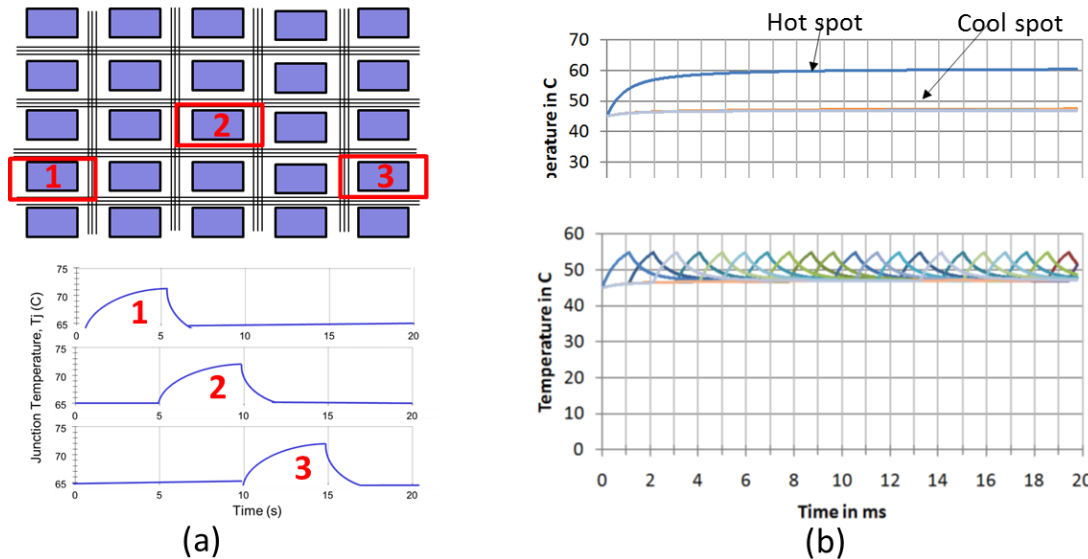
Figure 11: a) Illustration of FPGA junction temperature as a computing module is moved from location 1 to 2 to 3, migration is triggered based on temperature reaching a specified threshold, b) “HotSpot” based simulation results, showing about a 5 degree decrease in maximum hot spot temperature, as compared to a design with a static layout [17].
