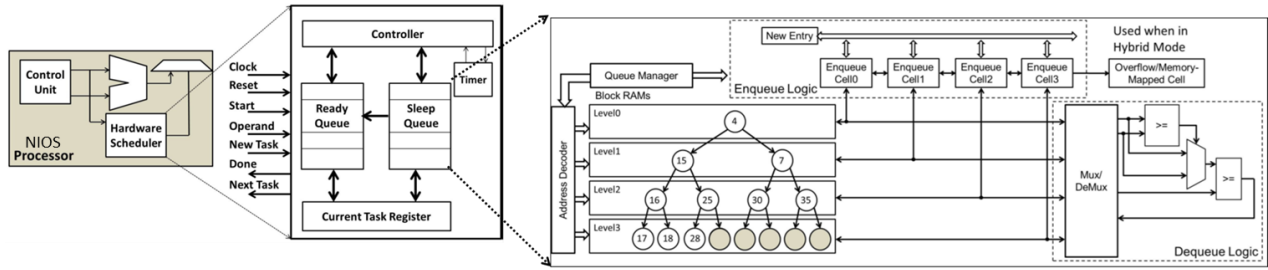
(a) SW/Hardware co-design of a Priority Queue implemented as a custom instruction
