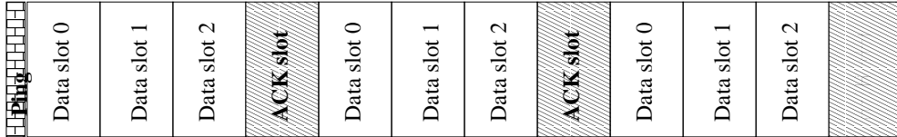
Fig. 4: Data and acknowledgement slots once synchronization is established.
