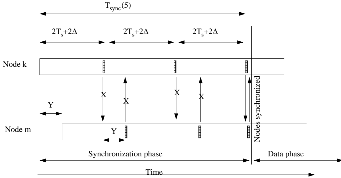
Fig. 8: Synchronization phase in S-MAC. Y represents the absolute difference between the wake up times of the sender and receiver nodes.
