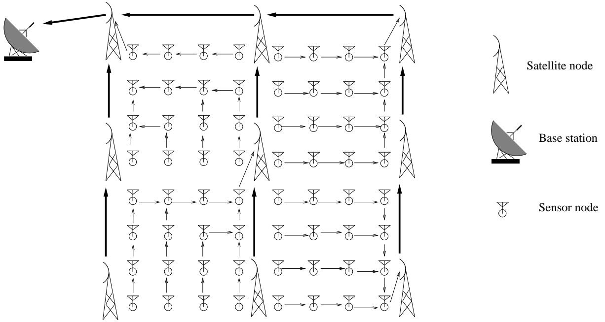
Fig. 1: Wireless sensor network, showing sensor and satellite station deployments and our hierarchical routing strategy.
