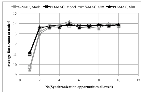
Fig. 7: Expected data count stored at sink.
