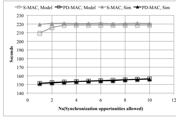
Fig. 9: Expected round duration vs. number of synchronization opportunities.
