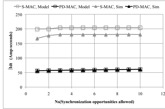
Fig. 10: Expected energy consumption per node.
