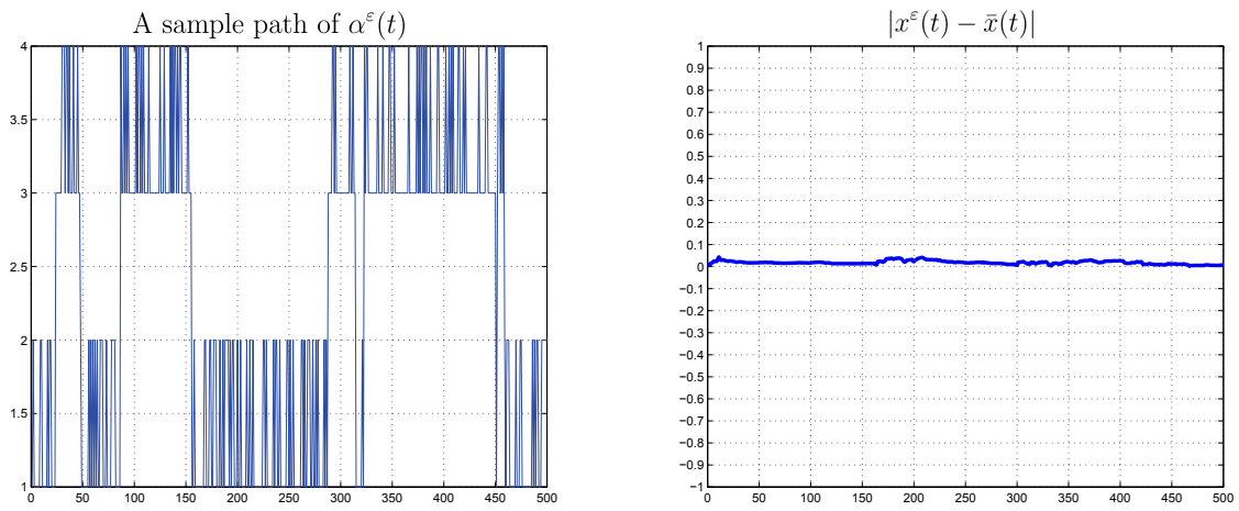
Figure 2: Sample path with \varepsilon = 0.01 in Example 5.6
