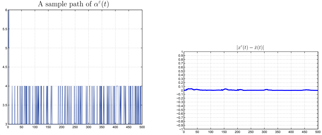
Figure 4: Sample path with \varepsilon = 0.01 in Example 5.7
