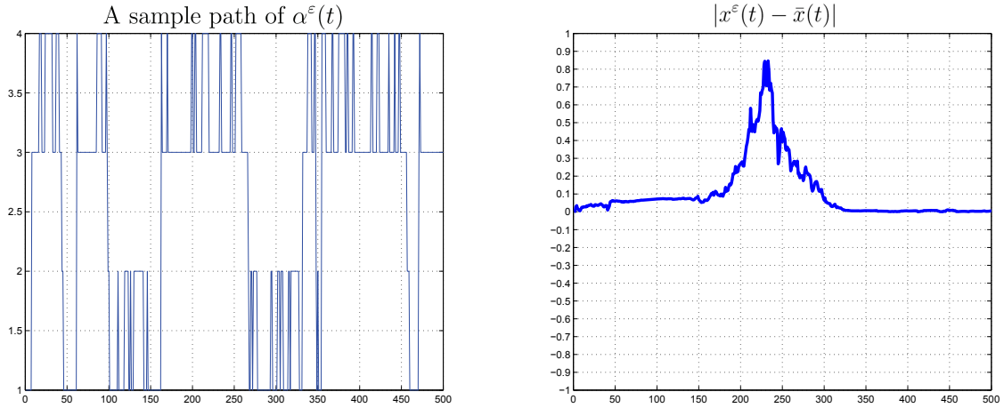
Figure 1: Sample path with \varepsilon = 0.1 in Example 5.6
