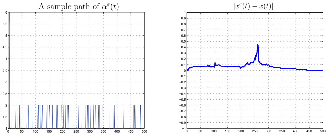
Figure 3: Sample path with \varepsilon = 0.1 in Example 5.7
