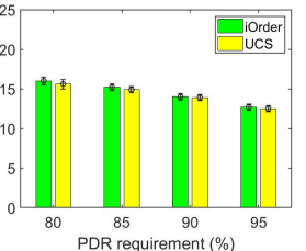
Fig. 28. Comparison with iOrder under the grid topology
