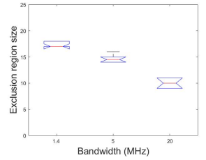
Fig. 18. Exclusion region size for different bandwidth
