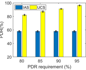
Fig. 25. Predictable reliability guarantee comparison with IAS
