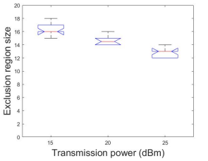
Fig. 22. Exclusion region size in heterogeneous power scenario
