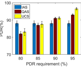
Fig. 23. Predictable reliability guarantee for random topology
