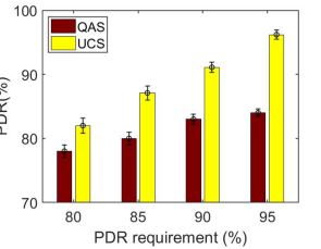
Fig. 26. Predictable reliability guarantee comparison with QAS
