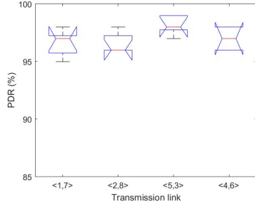
Fig. 9. Communication reliability in multi-cell scenario
