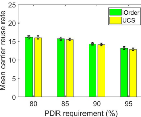
Fig. 27. Comparison with iOrder under the random topology
