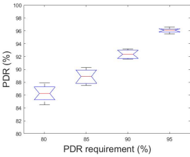
Fig. 19. Communication reliability in heterogeneous reliability scenario
