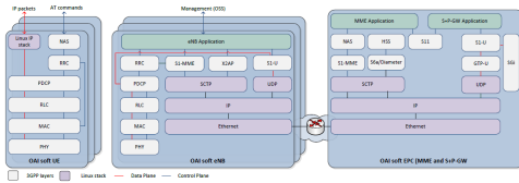
Fig. 3. The OpenAirInterface protocol stack
