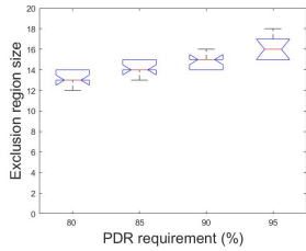
Fig. 20. Exclusion region size in heterogeneous reliability scenario
