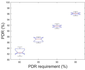
Fig. 21. Communication reliability in heterogeneous power scenario
