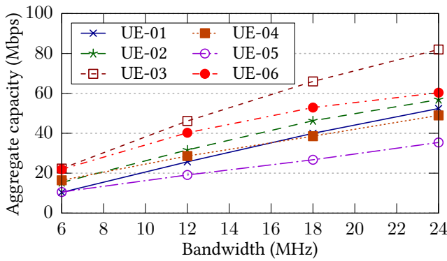
Figure 10: Aggregate Capacity (UL + DL) for Each UE
