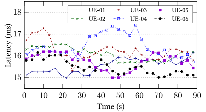
Figure 11: Latency between BS to UEs
