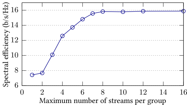
Figure 14: Impact of Increasing Spatial Streams on Spectral Efficiency
