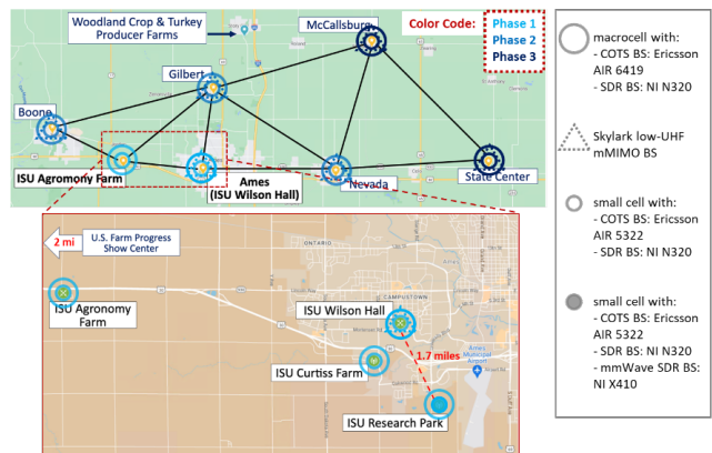
Figure 1: ARA PAWR Deployment
