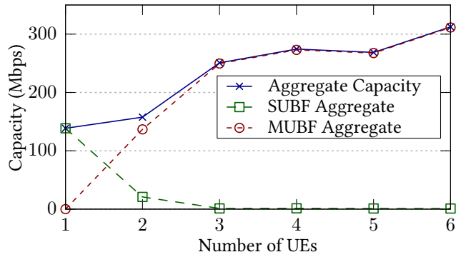
Figure 12: Impact of Number of UEs on System Capacity
